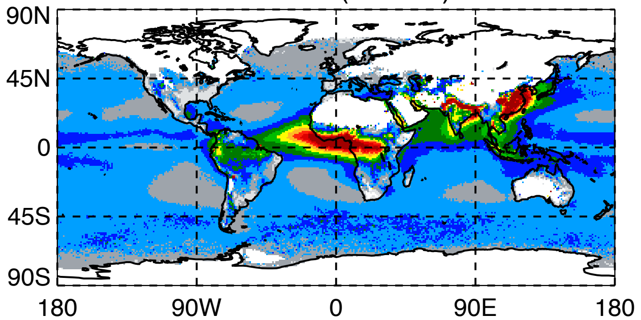
MODIS AOD (550nm) DJF
