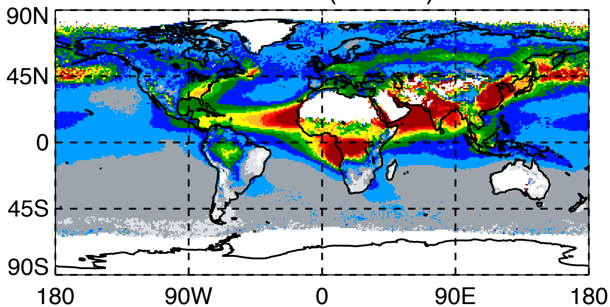
MODIS AOD (550nm) JJA
