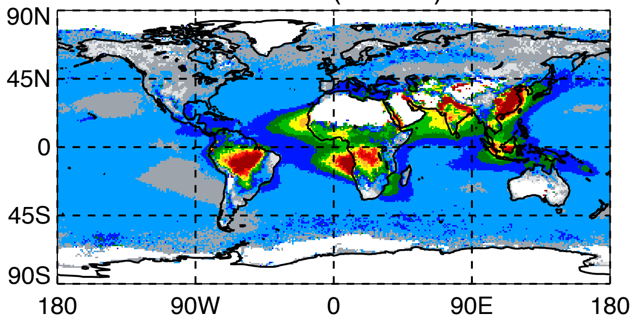
MODIS AOD (550nm) SON
