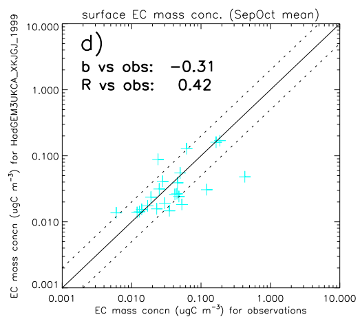
HadGEM3UKCA_XKJG_L1999 surface EC mass conc. (SepOct mean) ( \mu\text{gC m}^{-3} )
