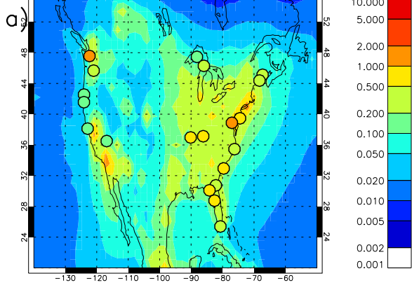
HadGEM3UKCA_XKJG_L1999 Annual mean EC mass conc. ( \mu\text{gC m}^{-3} )
