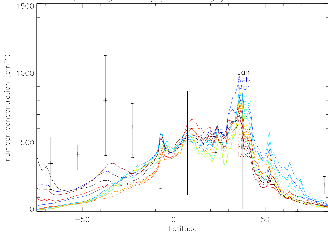
CN no. conc. (ocean gridboxes) (Heintz00Fig2): HadGEM3UKCA_XKJGJ_1999
