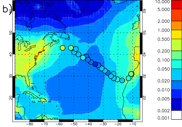
HadGEM3UKCA_XKJG_L1999 surface EC mass conc. (SepOct mean) ( \mu\text{gC m}^{-3} )
