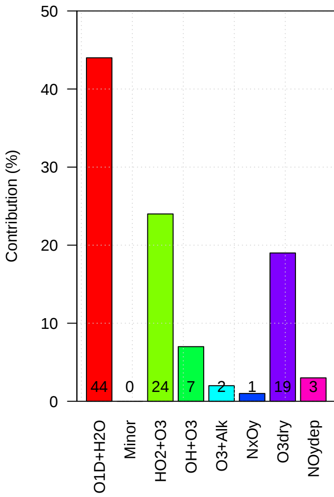
amekv Loss of Tropospheric Ox
