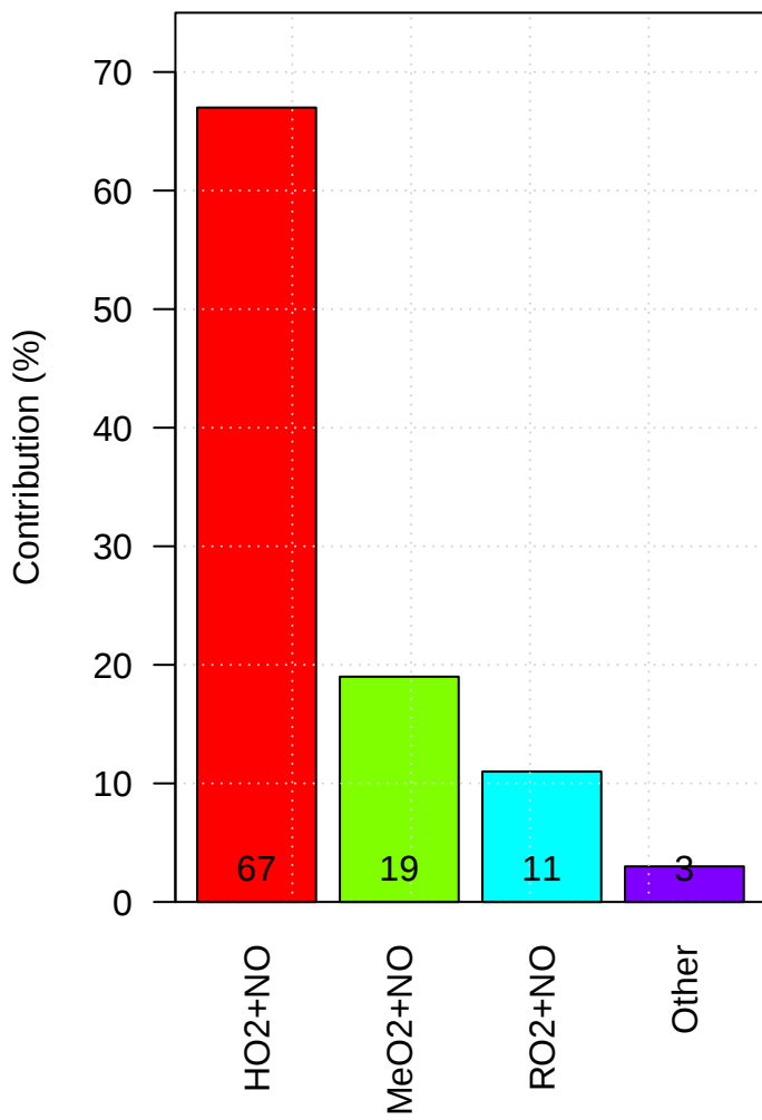
amekv Production of Tropospheric Ox
