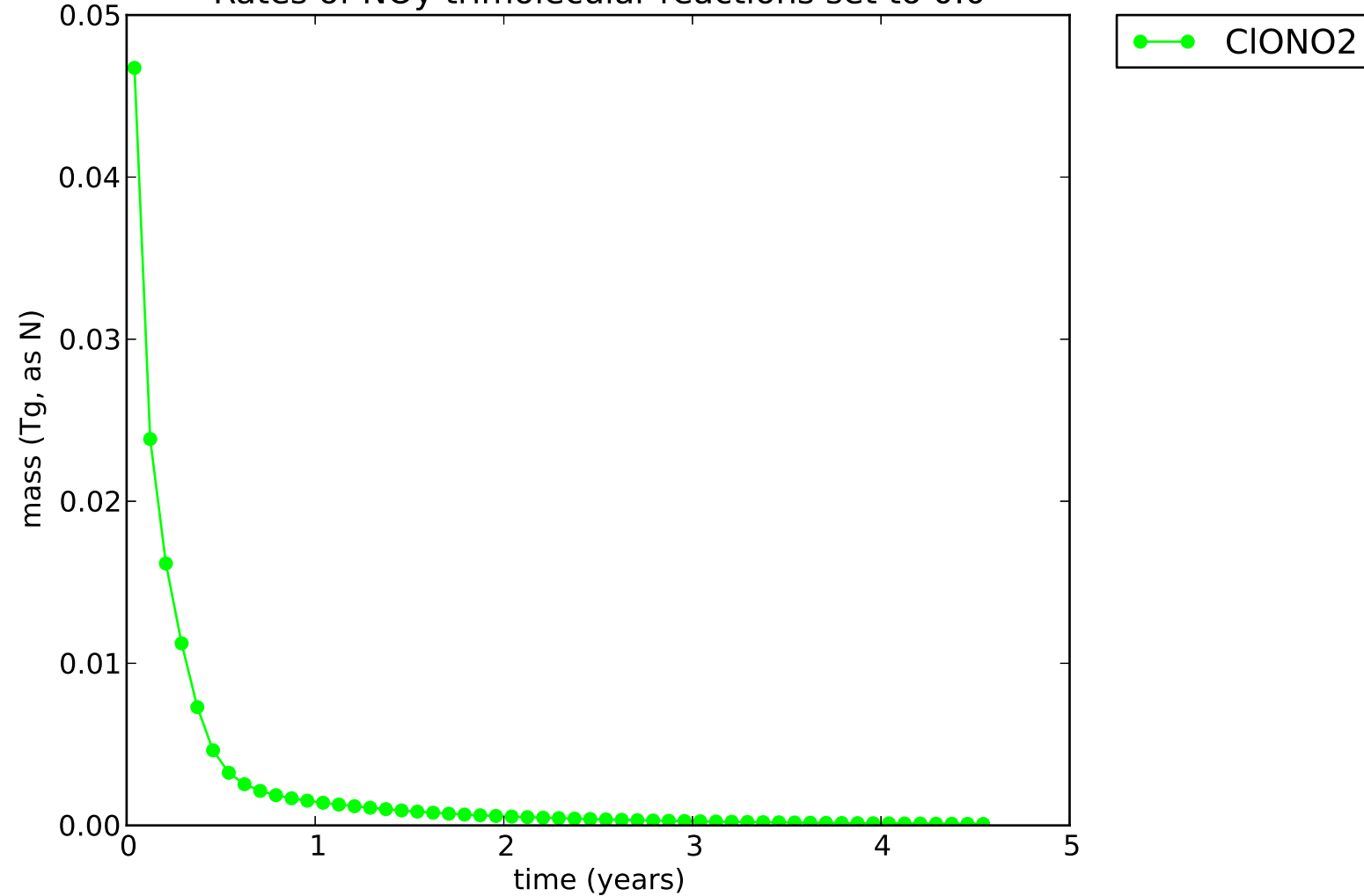
Rates of NOy trimolecular reactions set to 0.0
