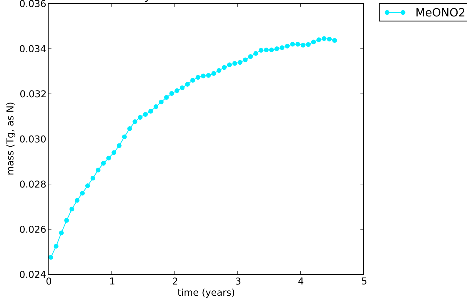
Rates of NOy trimolecular reactions set to 0.0
