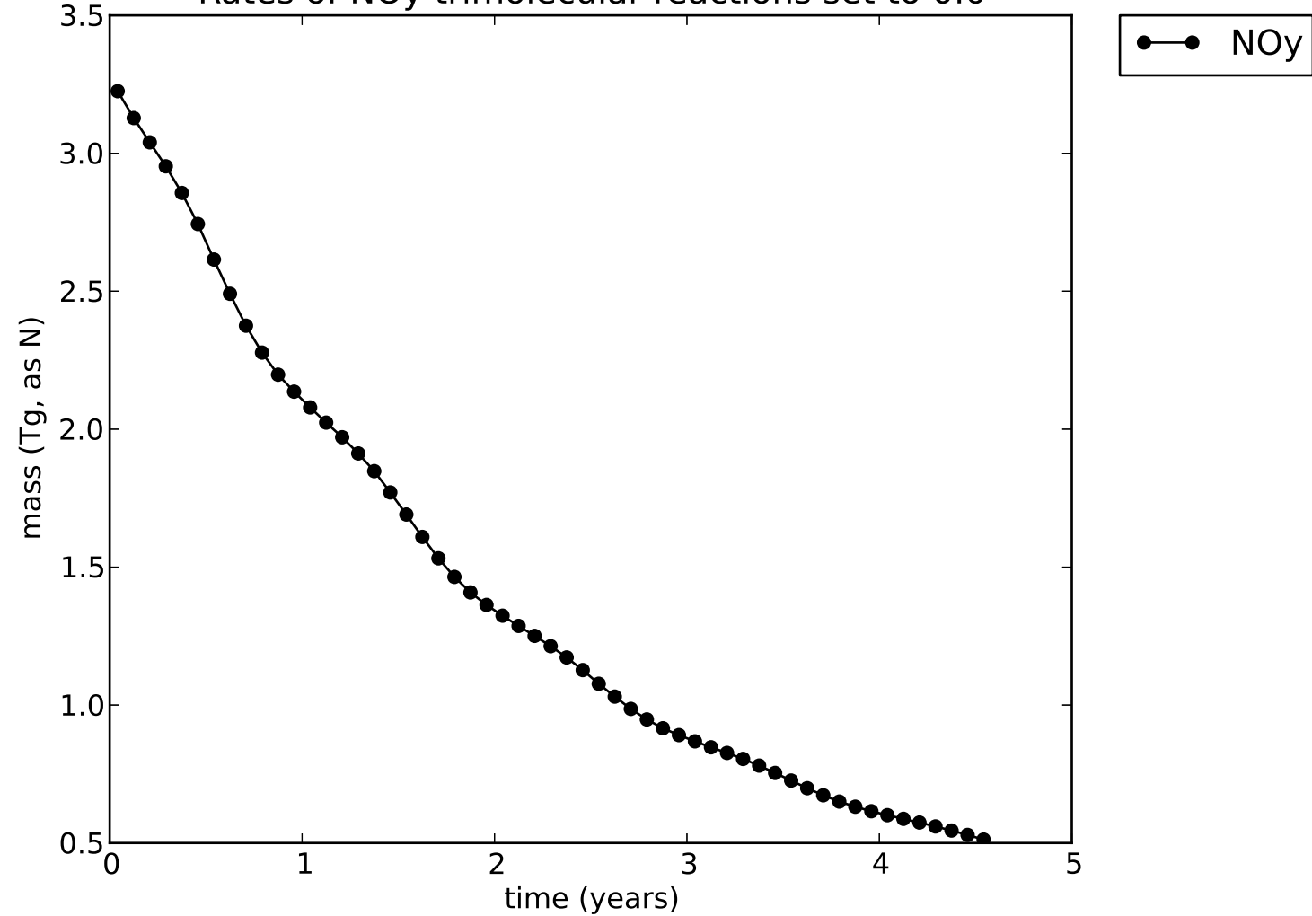
Rates of NOy trimolecular reactions set to 0.0
