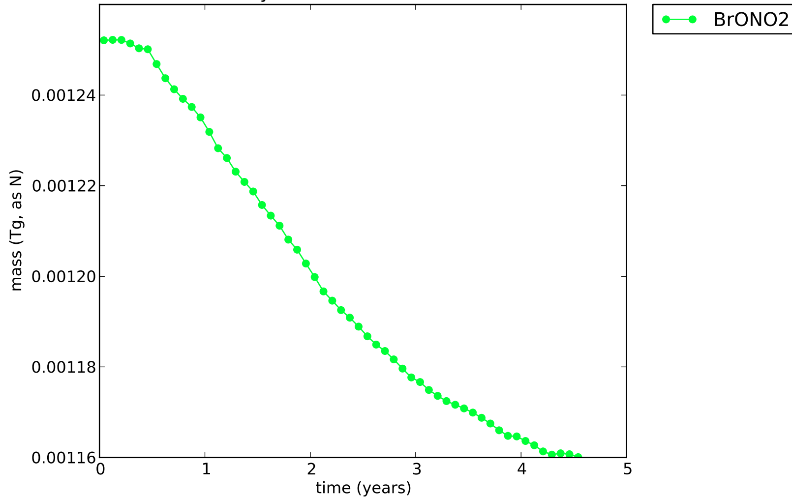
Rates of NOy trimolecular reactions set to 0.0
