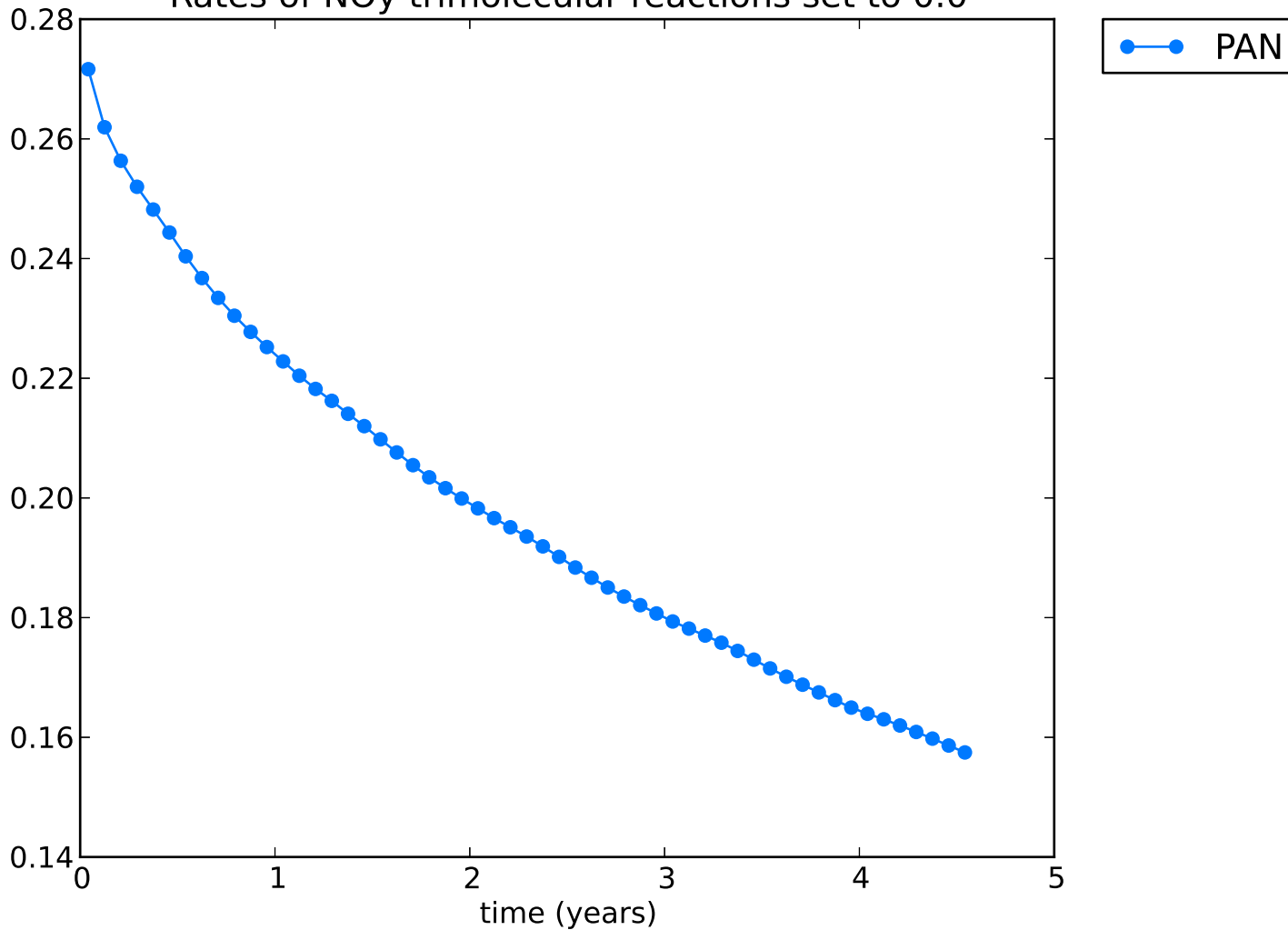
Rates of NOy trimolecular reactions set to 0.0
