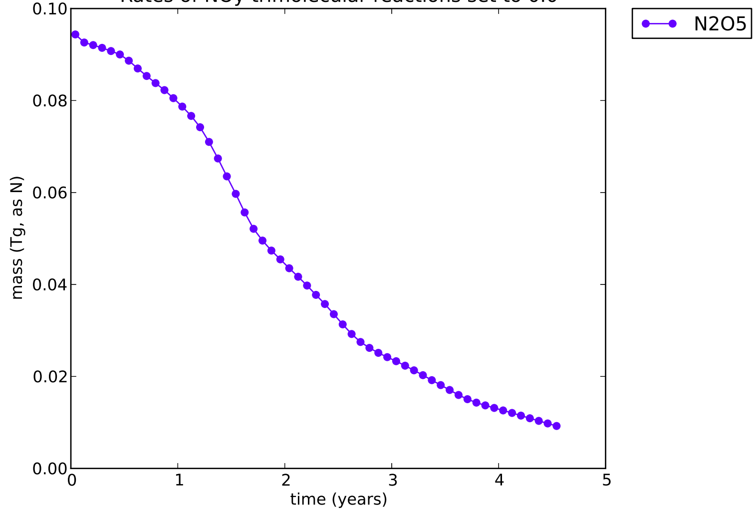
Rates of NOy trimolecular reactions set to 0.0
