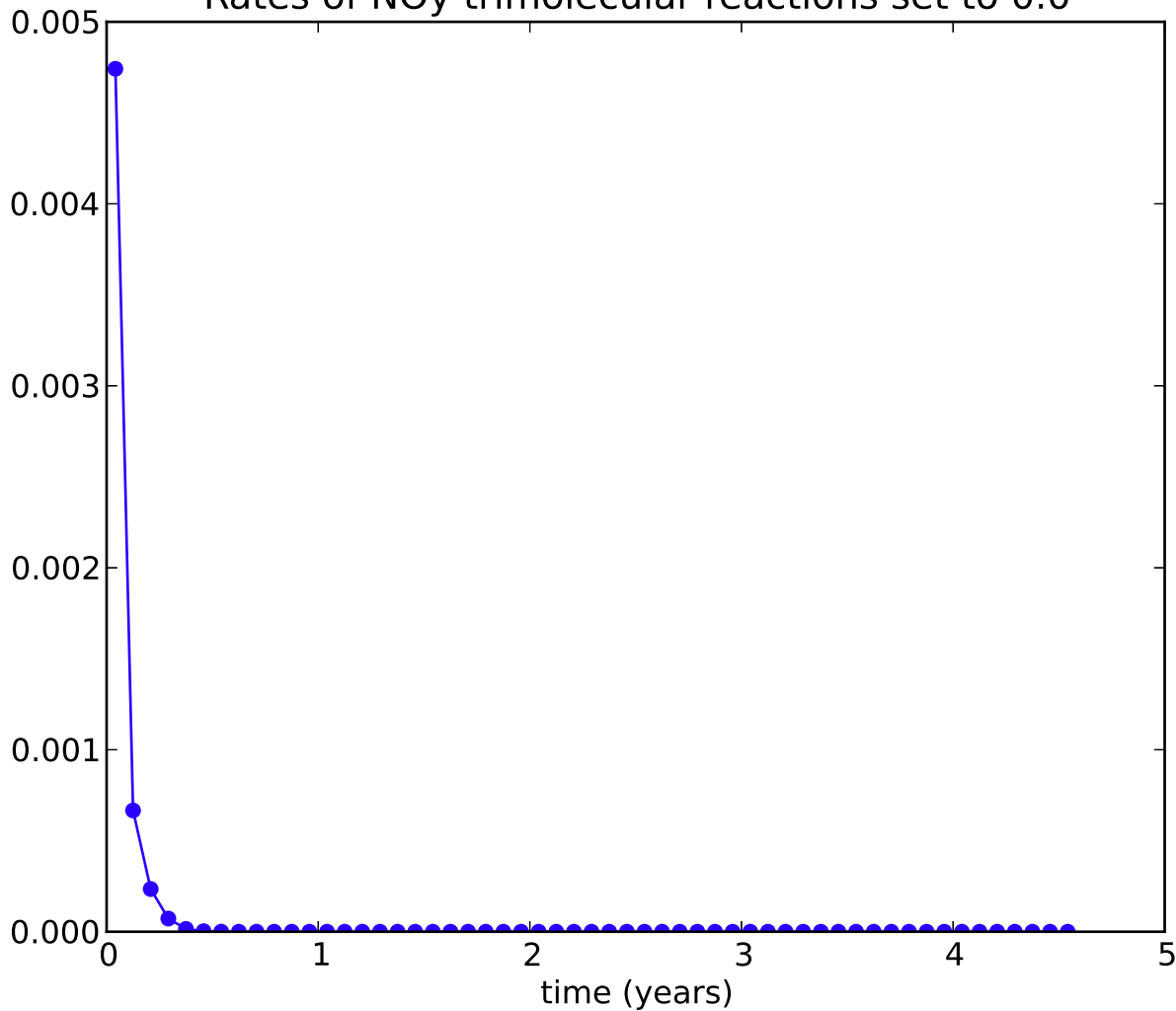
Rates of NOy trimolecular reactions set to 0.0
