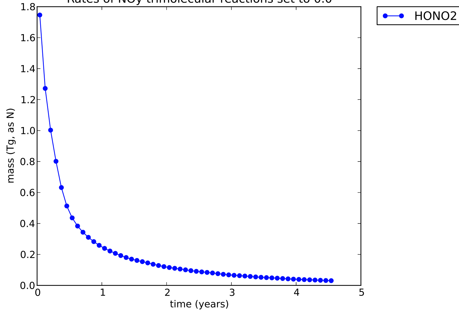
Rates of NO y trimolecular reactions set to 0.0
