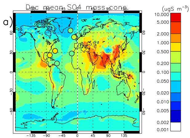
HadGEM3UKCA_BT692_2005 Vs EMEP,IMPROV,U.Miami
