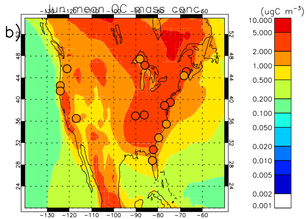
HadGEM3UKCA_BT692_2005 Vs IMPROVE 2000
