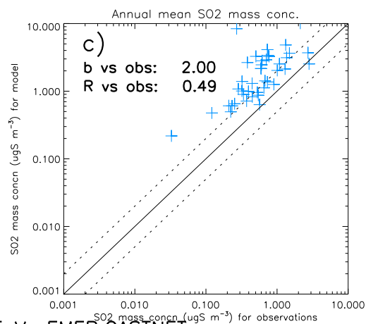
HadGEM3UKCA_BT692_2005 Vs EMEP,CASTNET
