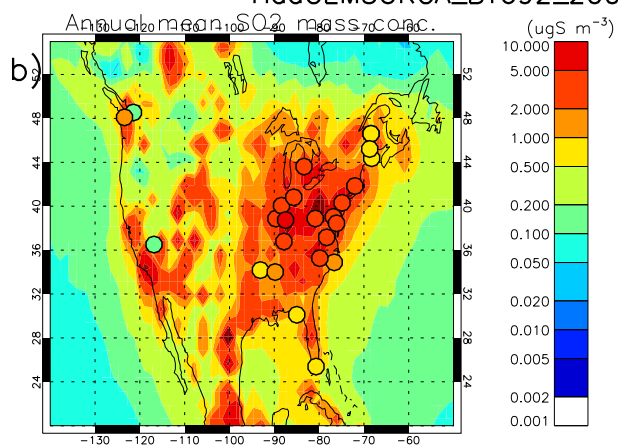
HadGEM3UKCA_BT692_2005 Vs EMEP,CASTNET
