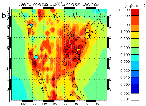
HadGEM3UKCA_BT692_2005 Vs EMEP,CASINET
