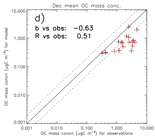
HadGEM3UKCA_BT692_2005 Vs IMPROVE 2000
