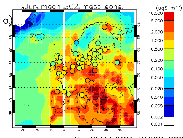
HadGEM3UKCA_BT692_2005 Vs EMEP,CASTNET
