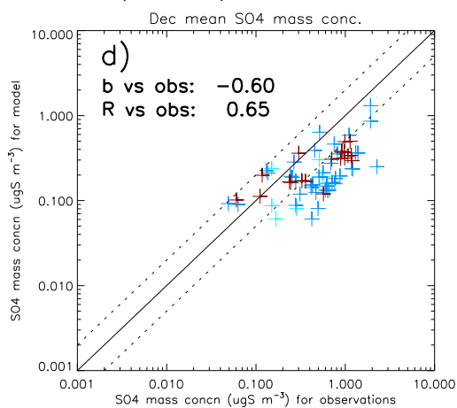
HadGEM3UKCA_BT692_2005 Vs EMEP,IMPROV,U.Miami
