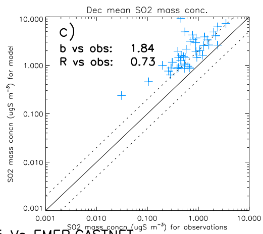
HadGEM3UKCA_BT692_2005 Vs EMEP,CASINET
