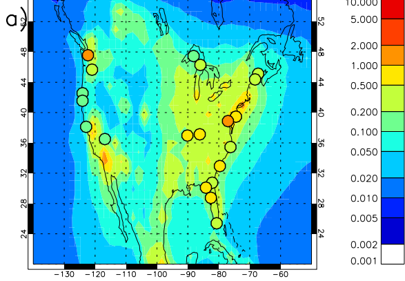
HadGEM3UKCA-XKAWA2006 Annual mean EC mass conc. ( \mu\text{gC m}^{-3} )
