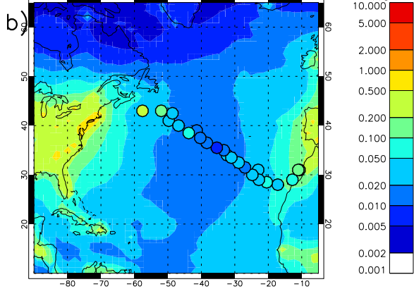
HadGEM3UKCA-XKAWA2006 surface EC mass conc. (SepOct mean) ( \mu\text{gC m}^{-3} )
