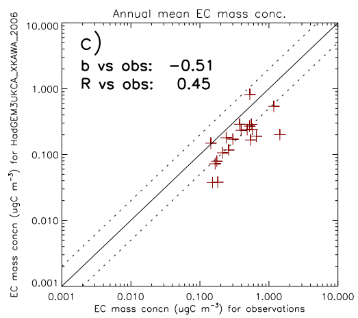
HadGEM3UKCA-XKAWA2006 Annual mean EC mass conc. ( \mu\text{gC m}^{-3} )
