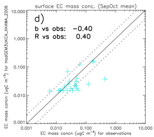
HadGEM3UKCA-XKAWA2006 surface EC mass conc. (SepOct mean) ( \mu\text{gC m}^{-3} )
