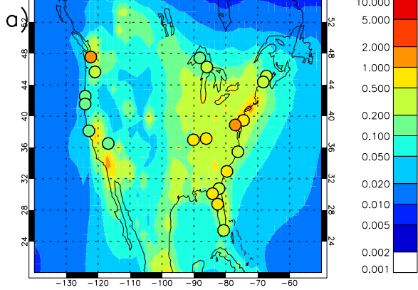
HadGEM3UKCA-XKAWA2003 Annual mean EC mass conc. ( \mu\text{gC m}^{-3} )
