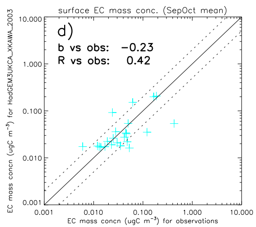
HadGEM3UKCA-XKAWA2003 surface EC mass conc. (SepOct mean) ( \mu\text{gC m}^{-3} )
