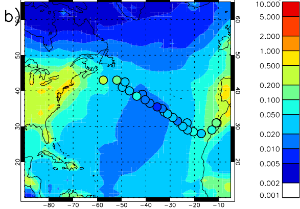
HadGEM3UKCA-XKAWA2003 surface EC mass conc. (SepOct mean) ( \mu\text{gC m}^{-3} )
