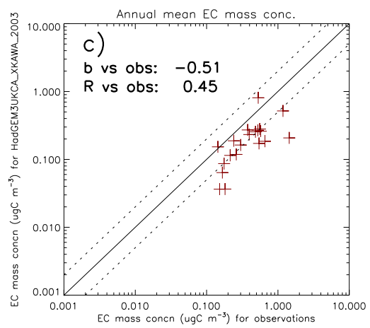
HadGEM3UKCA-XKAWA2003 Annual mean EC mass conc. ( \mu\text{gC m}^{-3} )
