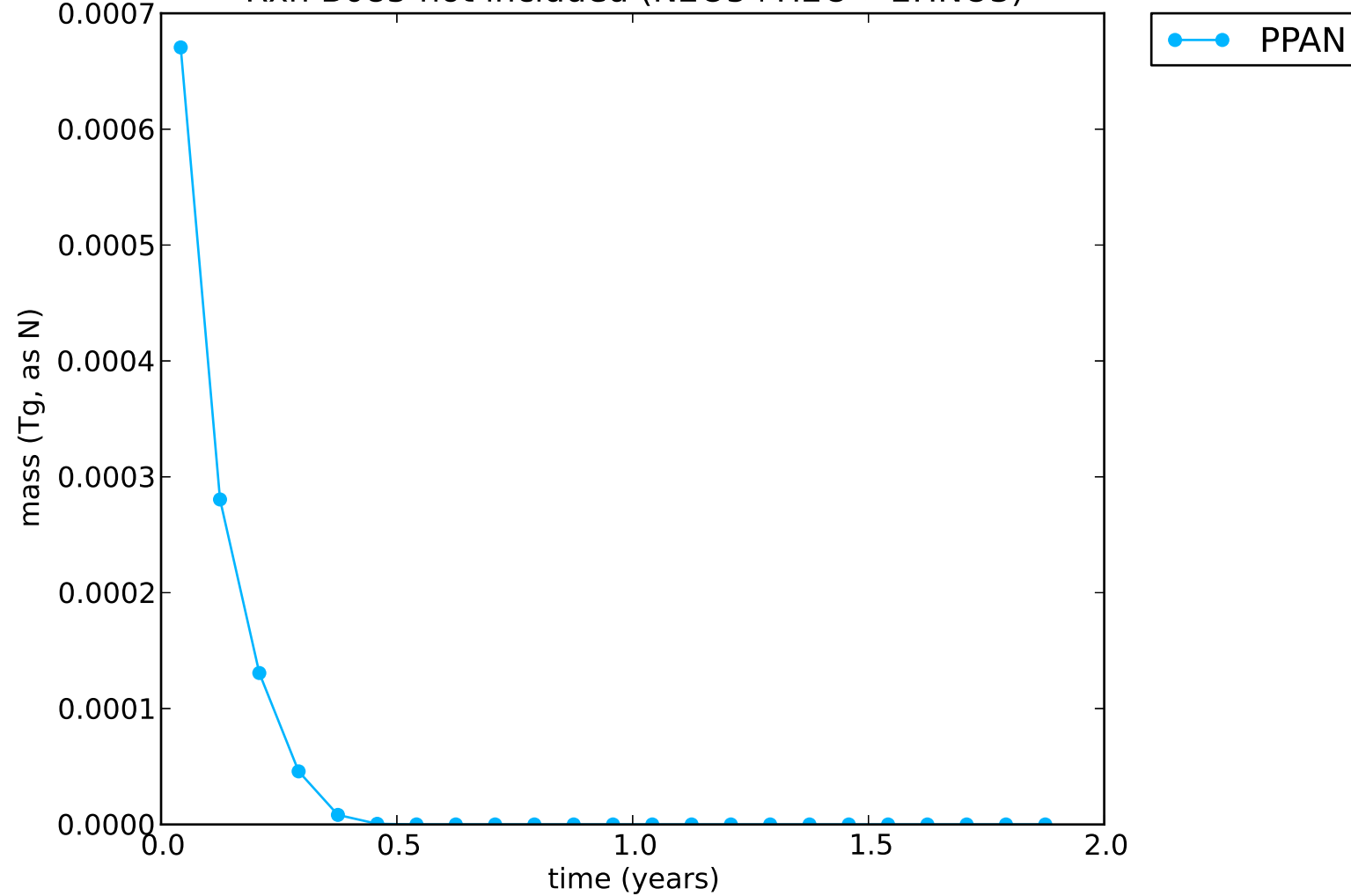
Rxn B085 not included ( \text{N}_2\text{O}_5 + \text{H}_2\text{O} \rightarrow 2\text{HNO}_3 )
