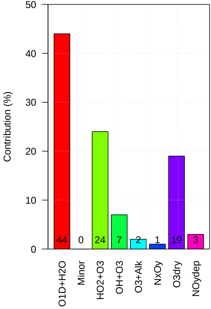
amekw Loss of Tropospheric Ox
