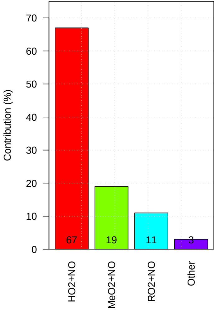
amekw Production of Tropospheric Ox
