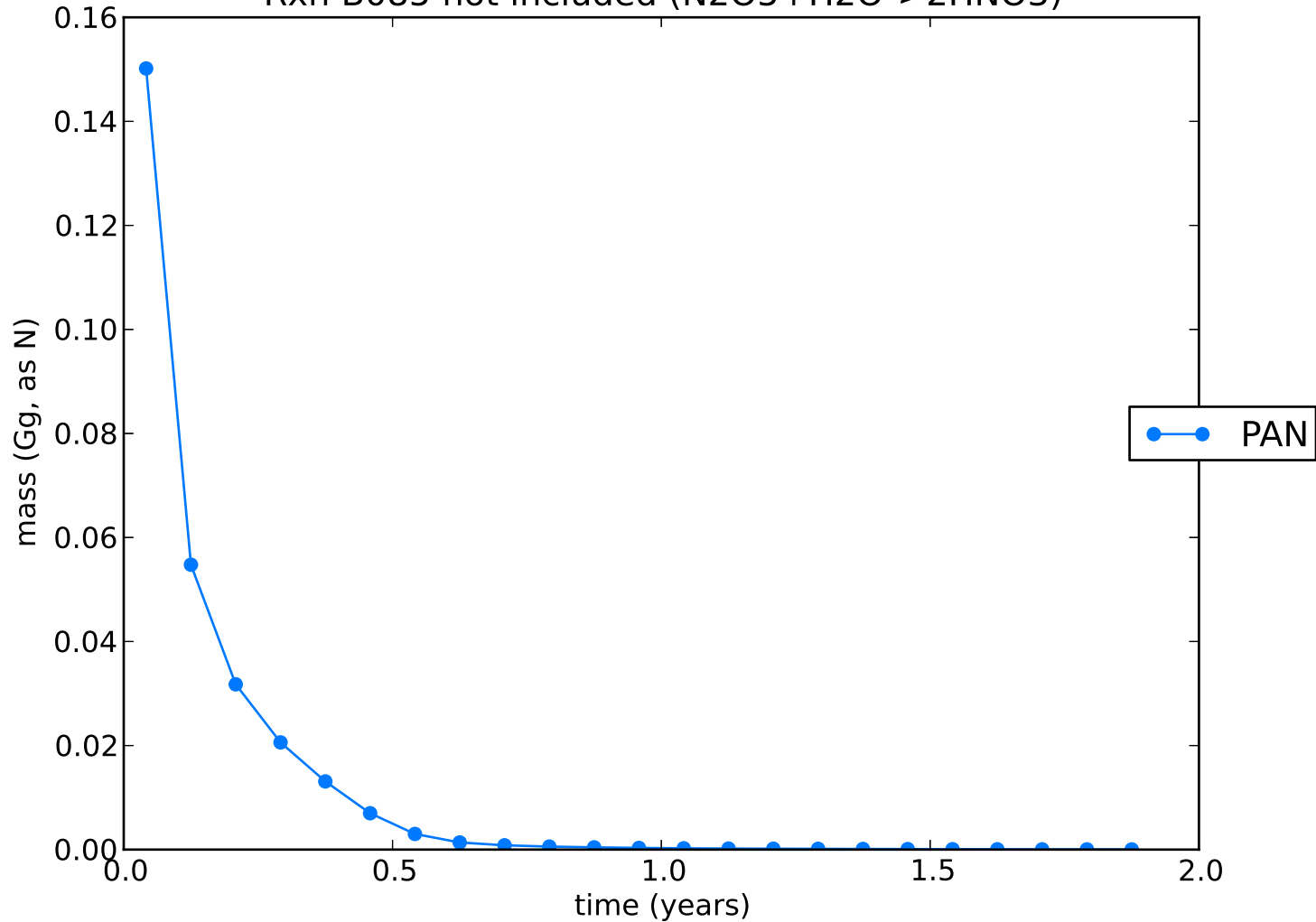
Rxn B085 not included ( \text{N}_2\text{O}_5 + \text{H}_2\text{O} \rightarrow 2\text{HNO}_3 )
