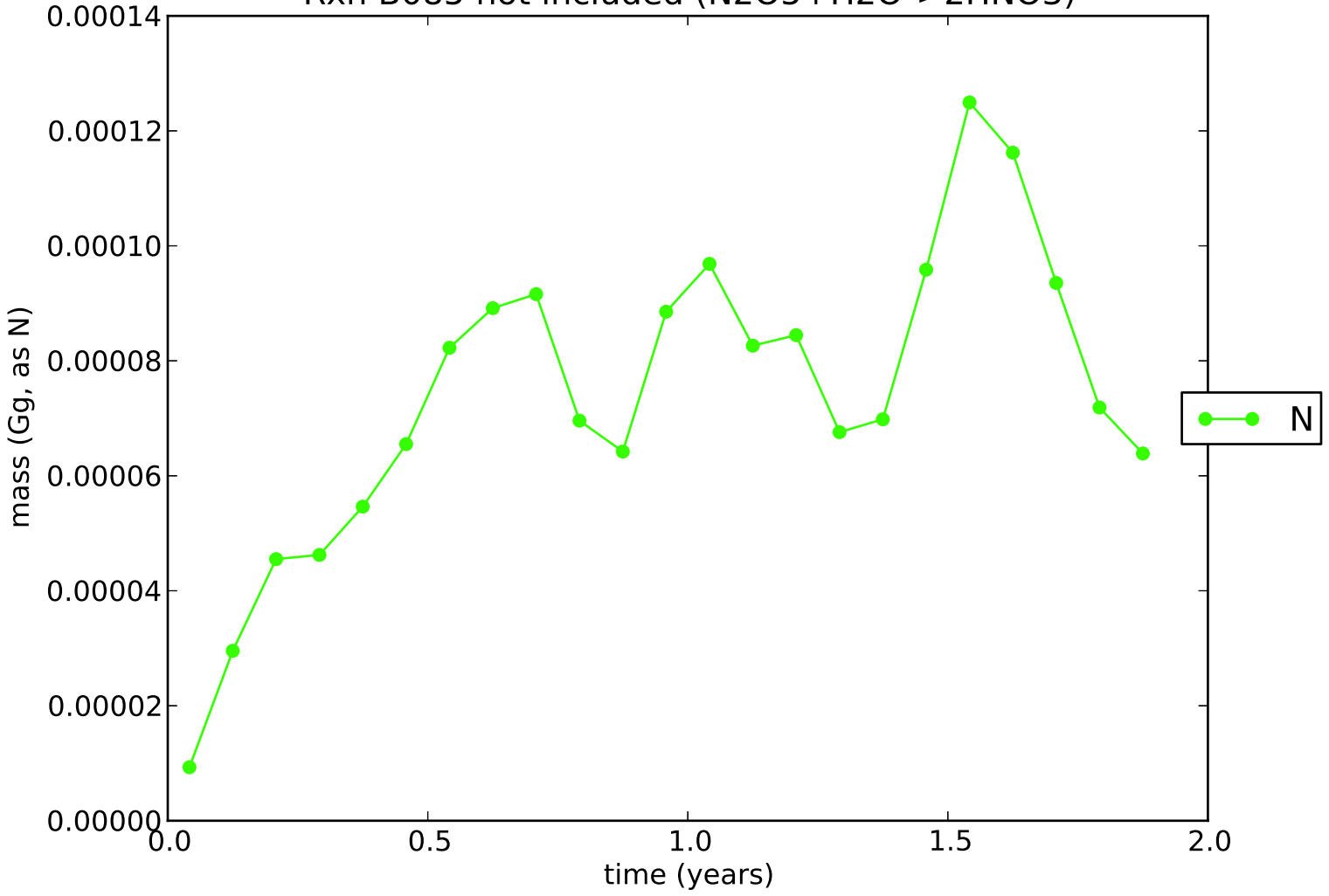
Rxn B085 not included (N2O5+H2O->2HNO3)
