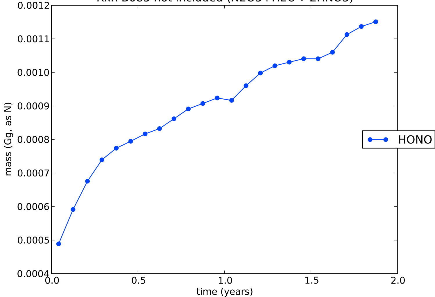
Rxn B085 not included (N2O5+H2O->2HNO3)
