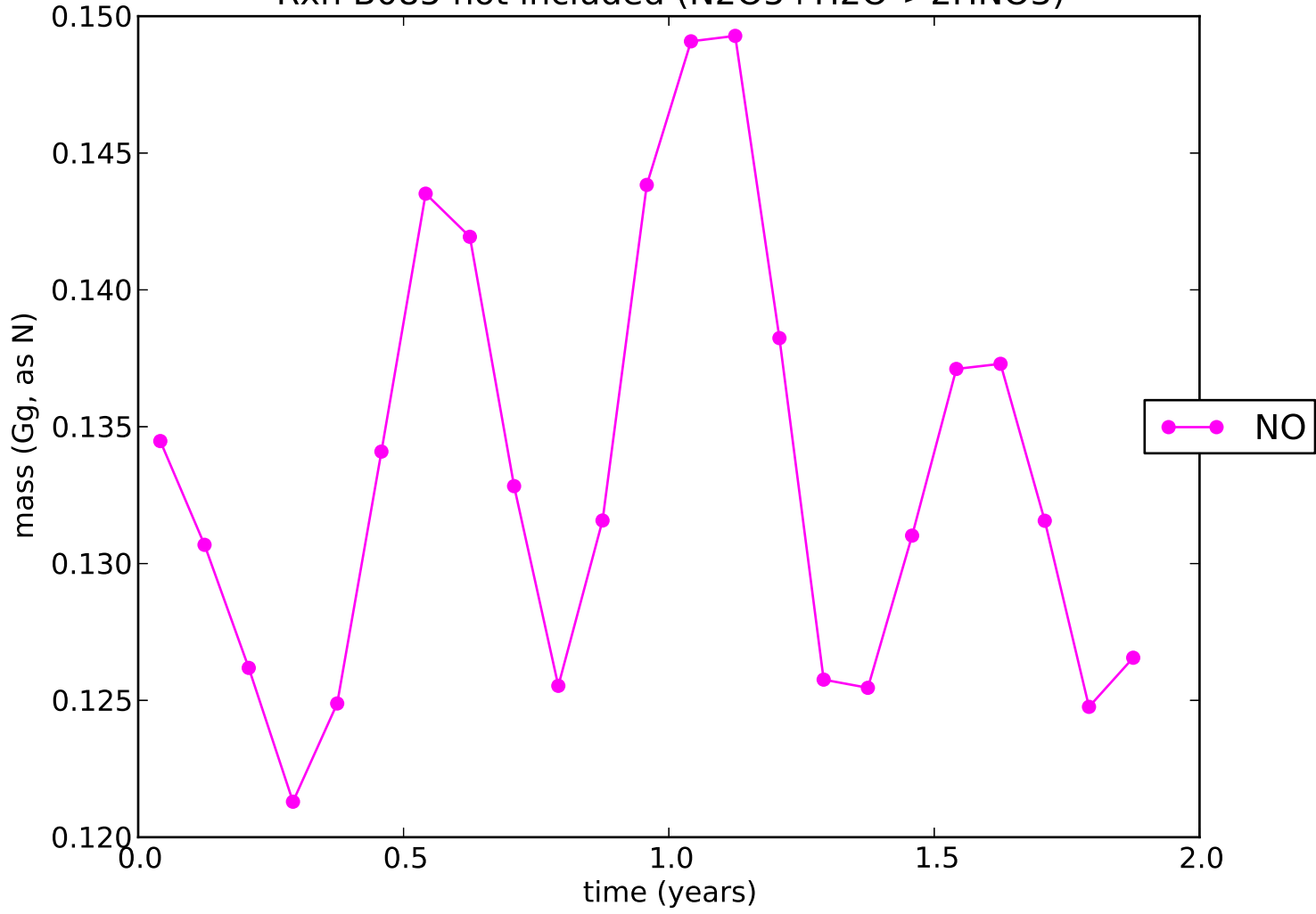
Rxn B085 not included (N2O5+H2O->2HNO3)
