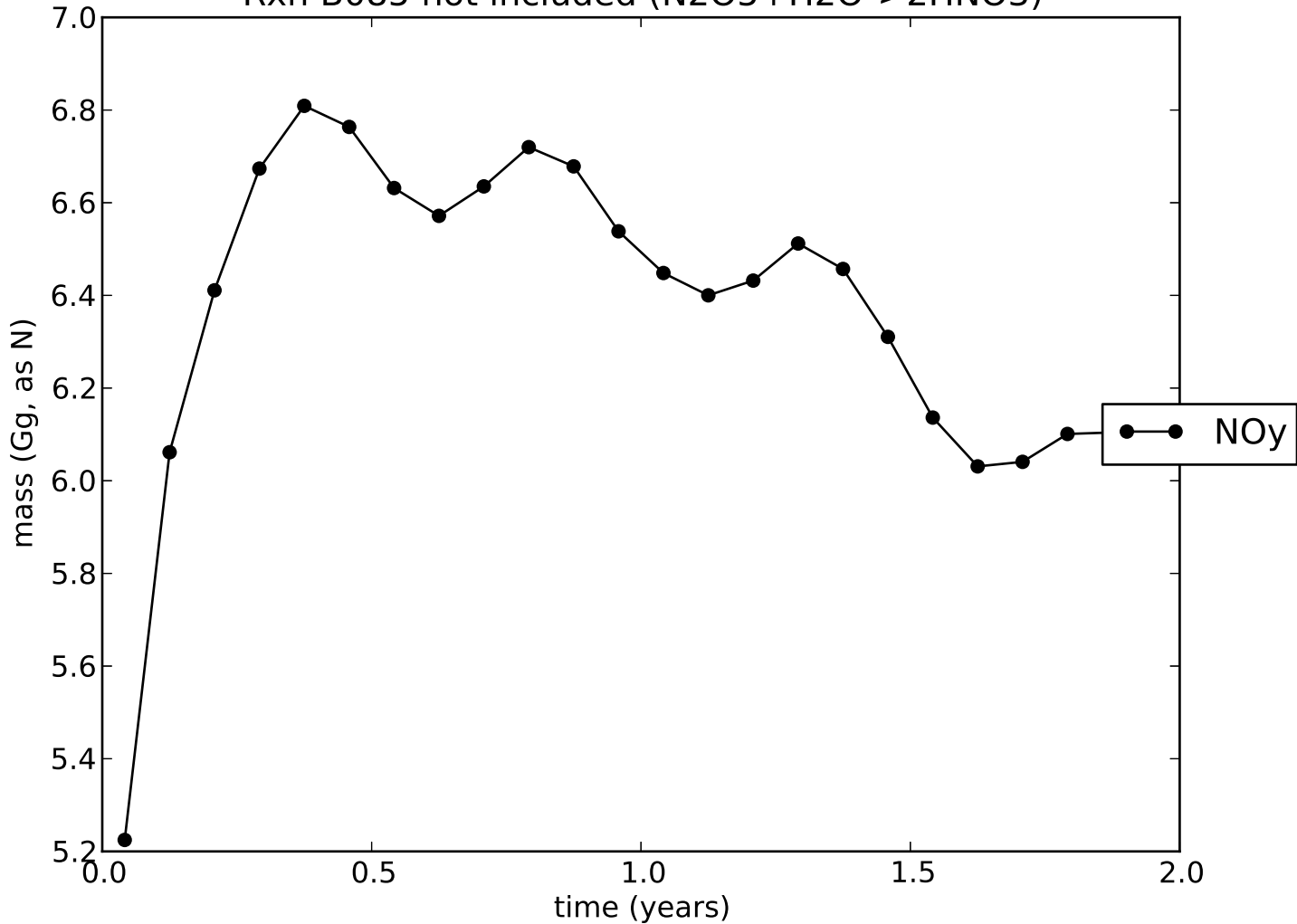
Rxn B085 not included (N2O5+H2O->2HNO3)
