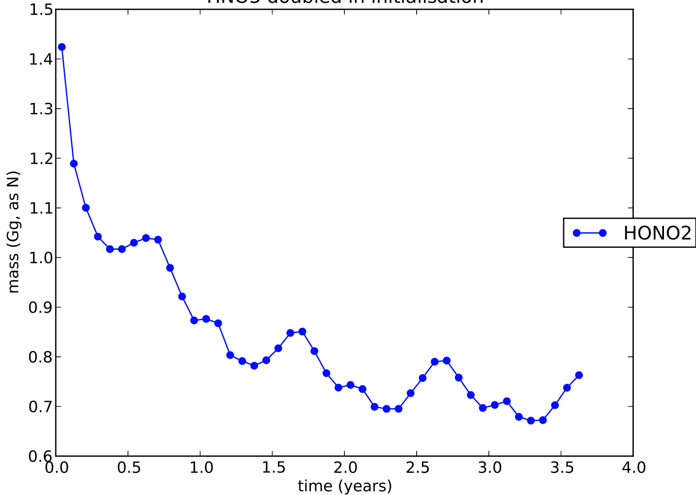
HNO3 doubled in initialisation
