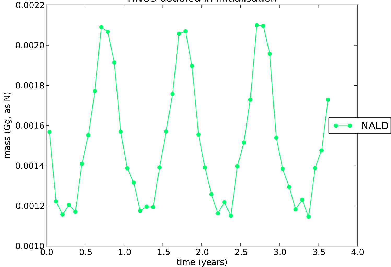
HNO3 doubled in initialisation
