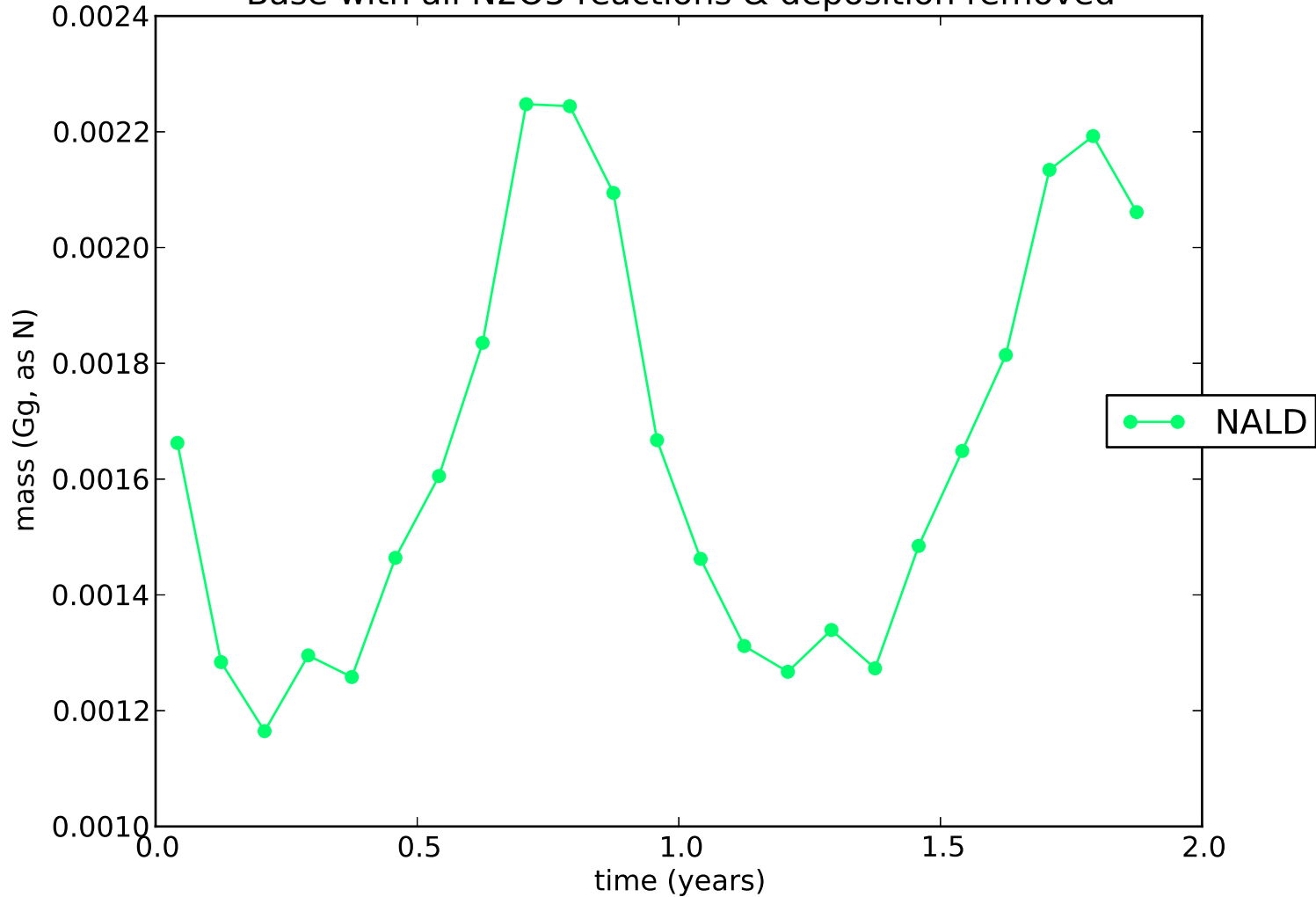
Base with all N2O5 reactions & deposition removed
