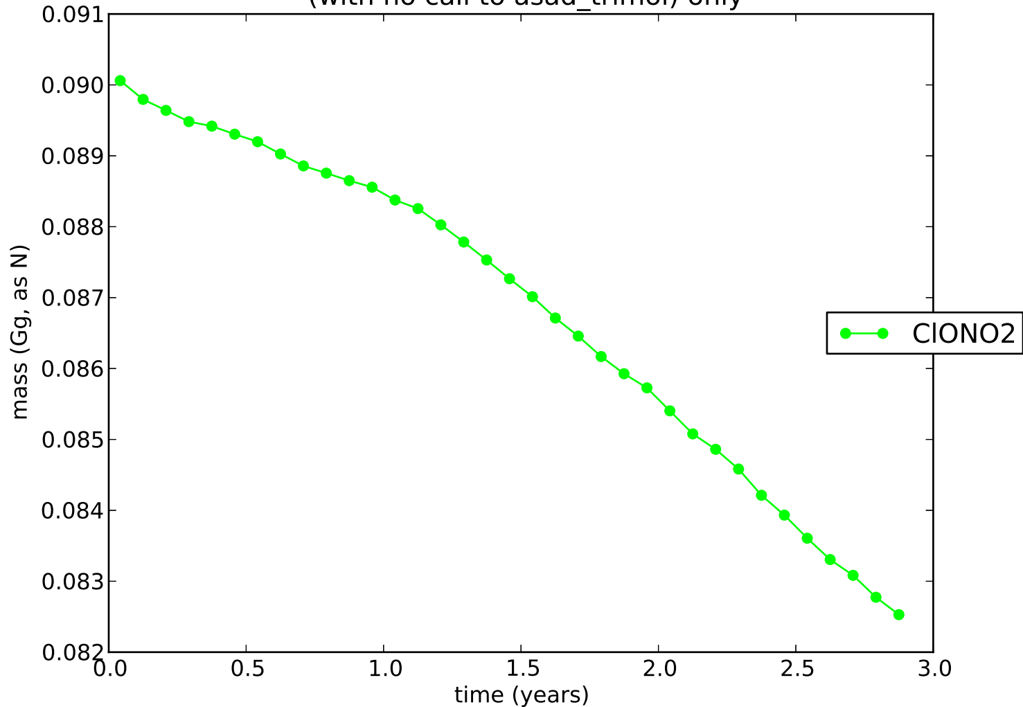
Call transform_halogen and chemistry_ctl (with no call to asad_trimol) only
