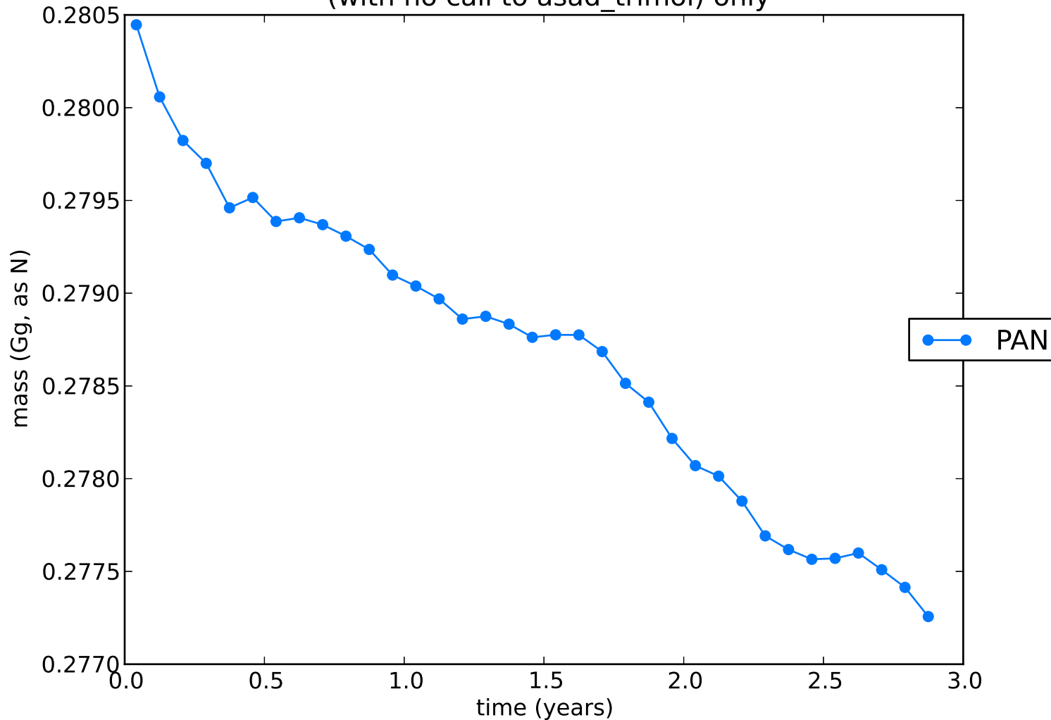
Call transform_halogen and chemistry_ctl (with no call to asad_trimol) only
