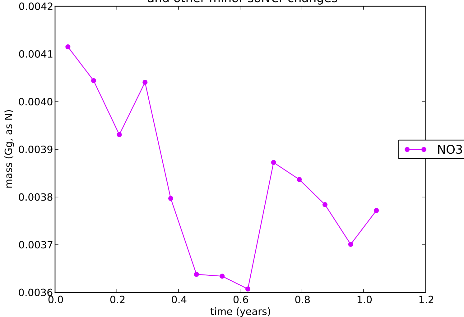
No prod/loss of NO y with 20min chemical timestep and other minor solver changes
