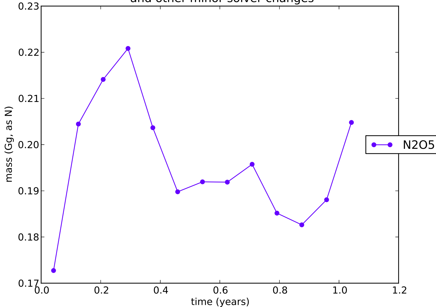
No prod/loss of NO y with 20min chemical timestep and other minor solver changes
