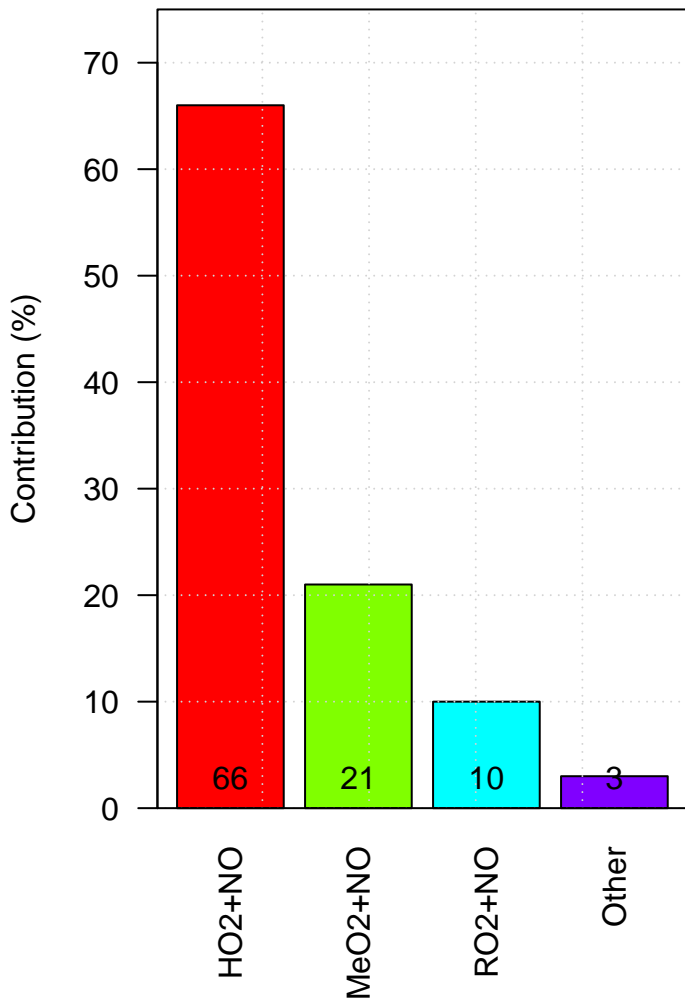
am400 Production of Tropospheric Ox
