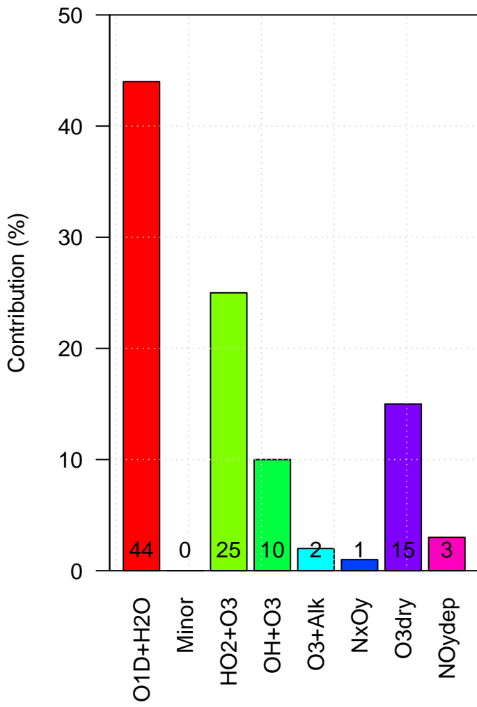
am400 Loss of Tropospheric Ox
