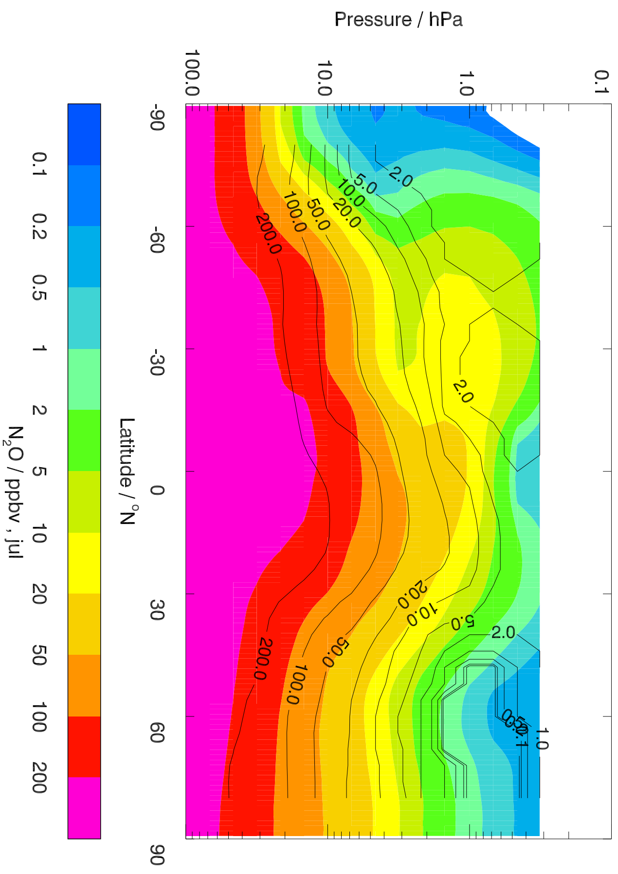
Colours: UKCA (XJGIN), Contours: HALOE
