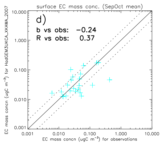
HadGEM3UKCA-XKAWA2007 surface EC mass conc. (SepOct mean) ( \mu\text{gC m}^{-3} )
