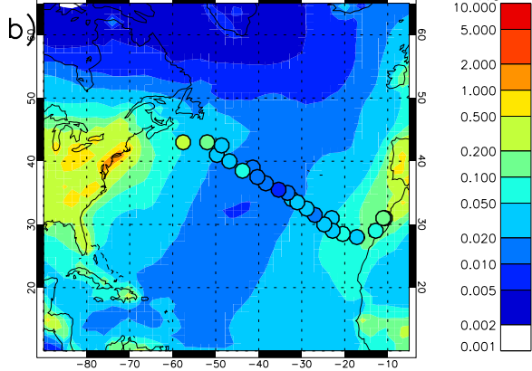
HadGEM3UKCA-XKAWA2007 surface EC mass conc. (SepOct mean) ( \mu\text{gC m}^{-3} )
