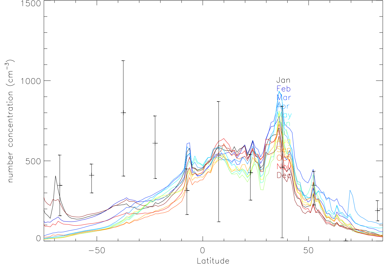
CN no. conc. (ocean gridboxes) (Heintz00Fig2): HadGEM3UKCA_XKAWA_2007
