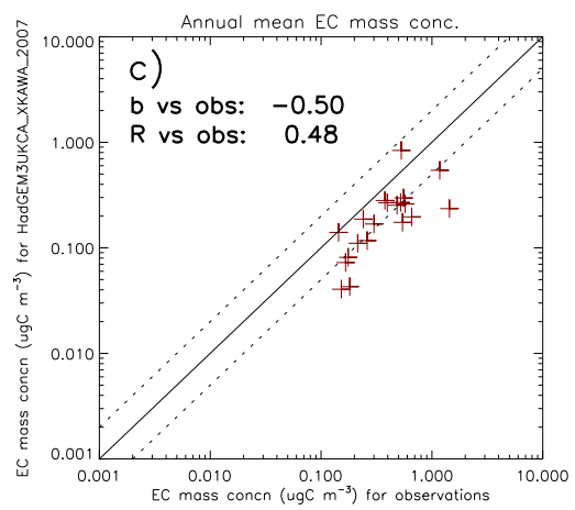
HadGEM3UKCA-XKAWA2007 Annual mean EC mass conc. ( \mu\text{gC m}^{-3} )
