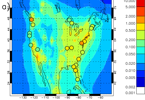
HadGEM3UKCA-XKAWA2007 Annual mean EC mass conc. ( \mu\text{gC m}^{-3} )
