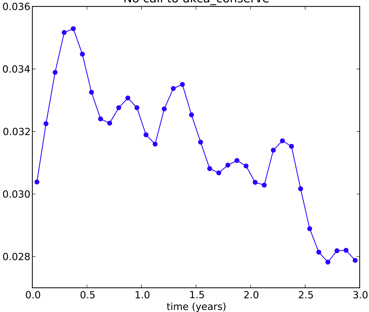
No call to ukca_conserve
