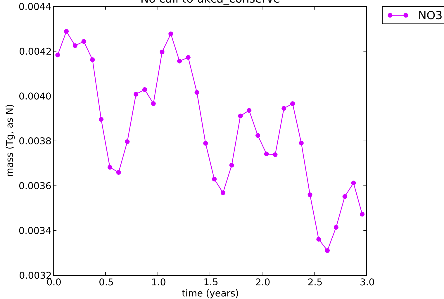
No call to ukca_conserve
