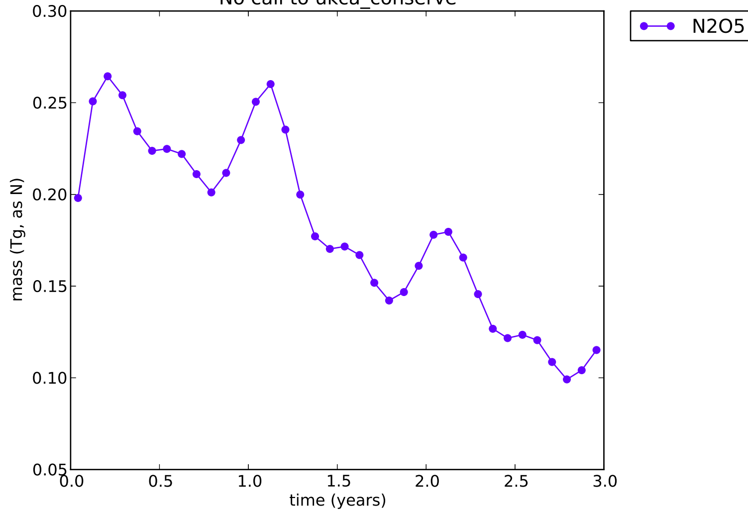
No call to ukca_conserve
