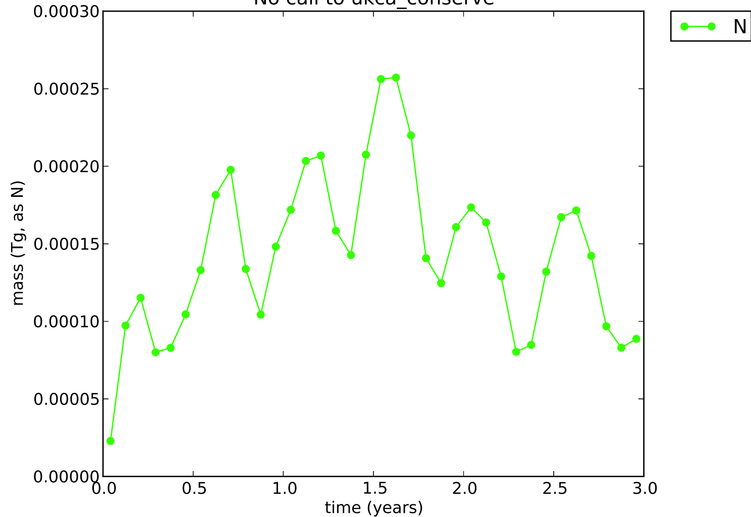
No call to ukca_conserve
