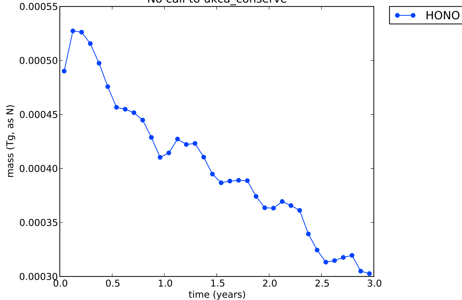
No call to ukca_conserve
