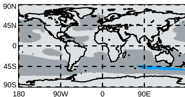
Coarse (Sol) AOD (440nm) GI: 0.039 NH: 0.023
