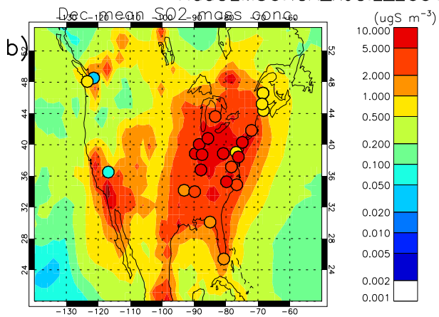
HadGEM3UKCA_XJCIL_2001 Vs EMEP,CASNET
