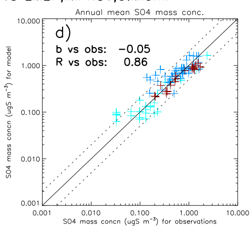
HadGEM3UKCA_XJCIL_2001 Vs EMEP, IMPROV, U.Miami
