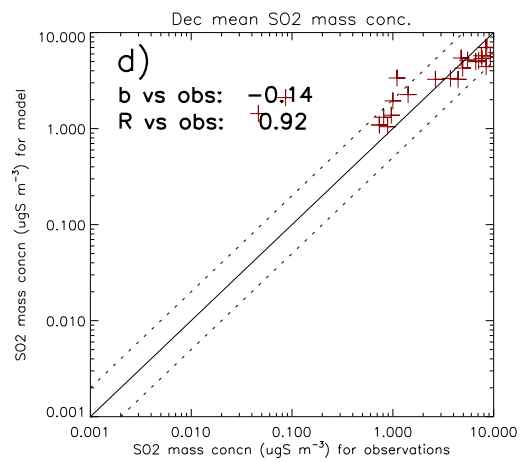
HadGEM3UKCA_XJCIL_2001 Vs EMEP,CASNET
