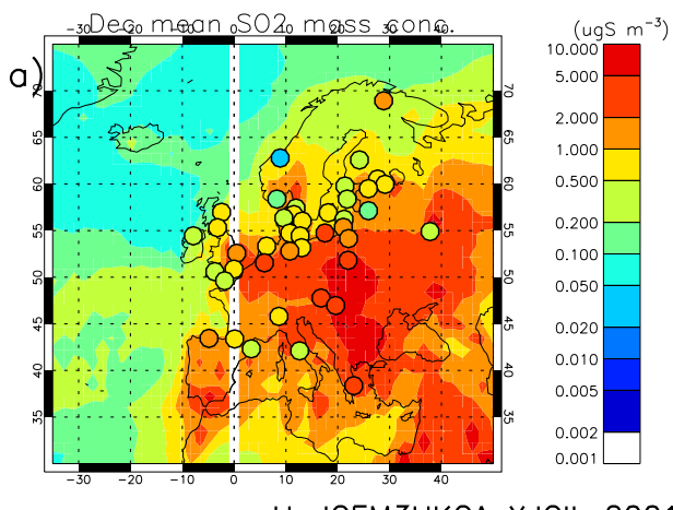
HadGEM3UKCA_XJCIL_2001 Vs EMEP,CASNET
