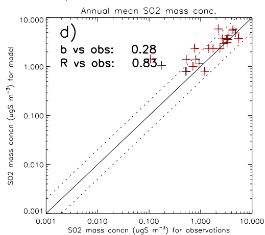
HadGEM3UKCA_XJCIL_2001 Vs EMEP,CASINET
