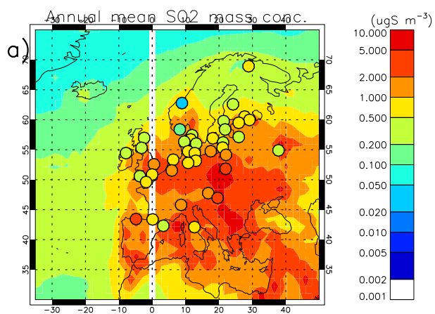
HadGEM3UKCA_XJCIL_2001 Vs EMEP,CASINET
