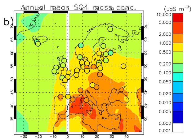
HadGEM3UKCA_XJCIL_2001 Vs EMEP, IMPROV, U.Miami
