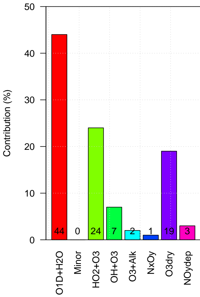
ameky Loss of Tropospheric Ox
