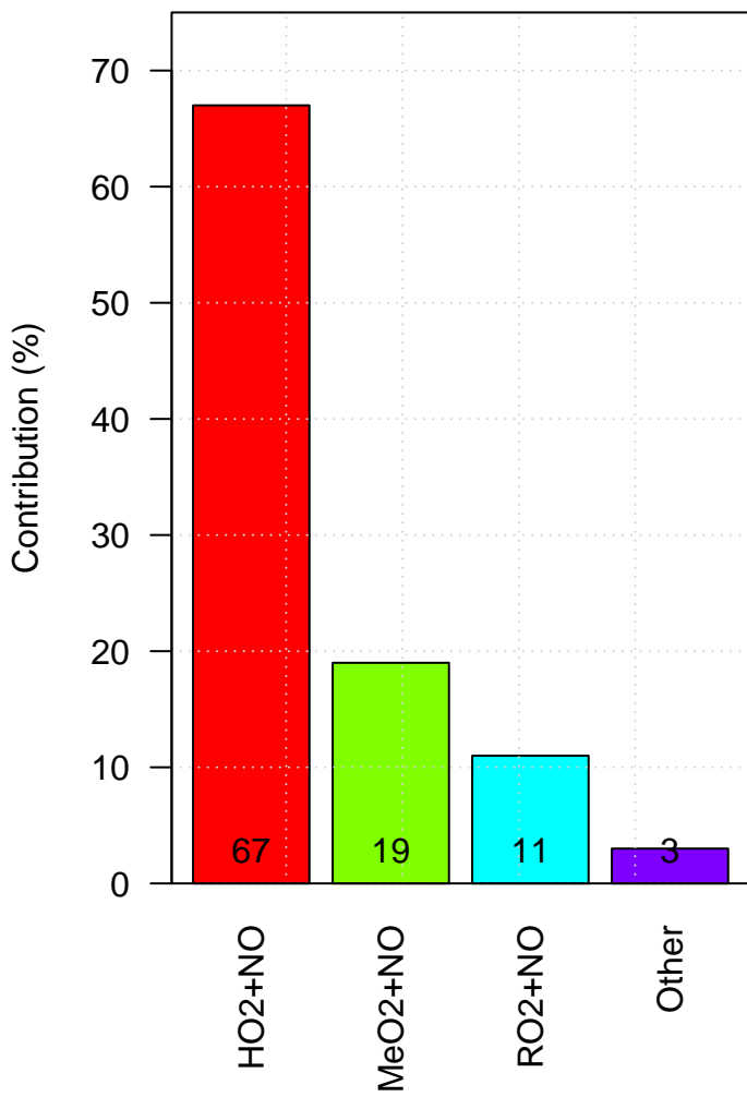
ameky Production of Tropospheric Ox
