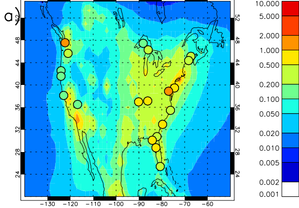
HadGEM3UKCA-XKAWA2005 Annual mean EC mass conc. ( \mu\text{gC m}^{-3} )
