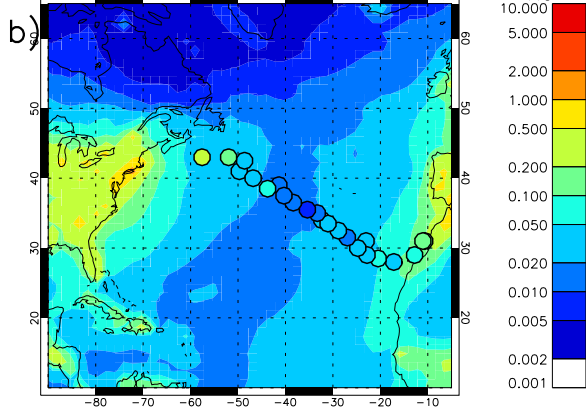
HadGEM3UKCA-XKAWA2005 surface EC mass conc. (SepOct mean) ( \mu\text{gC m}^{-3} )
