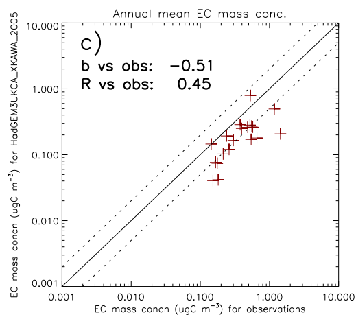
HadGEM3UKCA-XKAWA2005 Annual mean EC mass conc. ( \mu\text{gC m}^{-3} )
