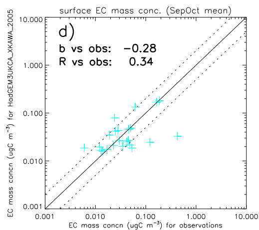
HadGEM3UKCA-XKAWA2005 surface EC mass conc. (SepOct mean) ( \mu\text{gC m}^{-3} )
