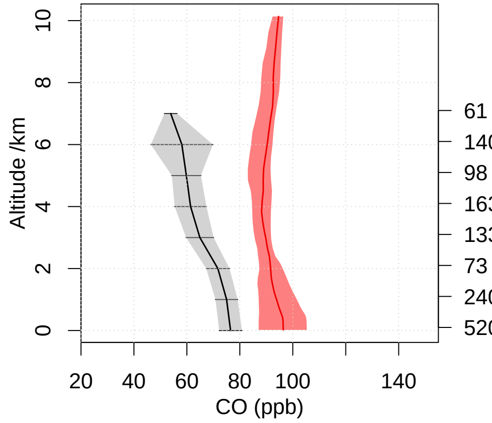
PEM-Tropics-B Christmas-Island 1999 C Lat 0 - 10 Lon 200 - 220
