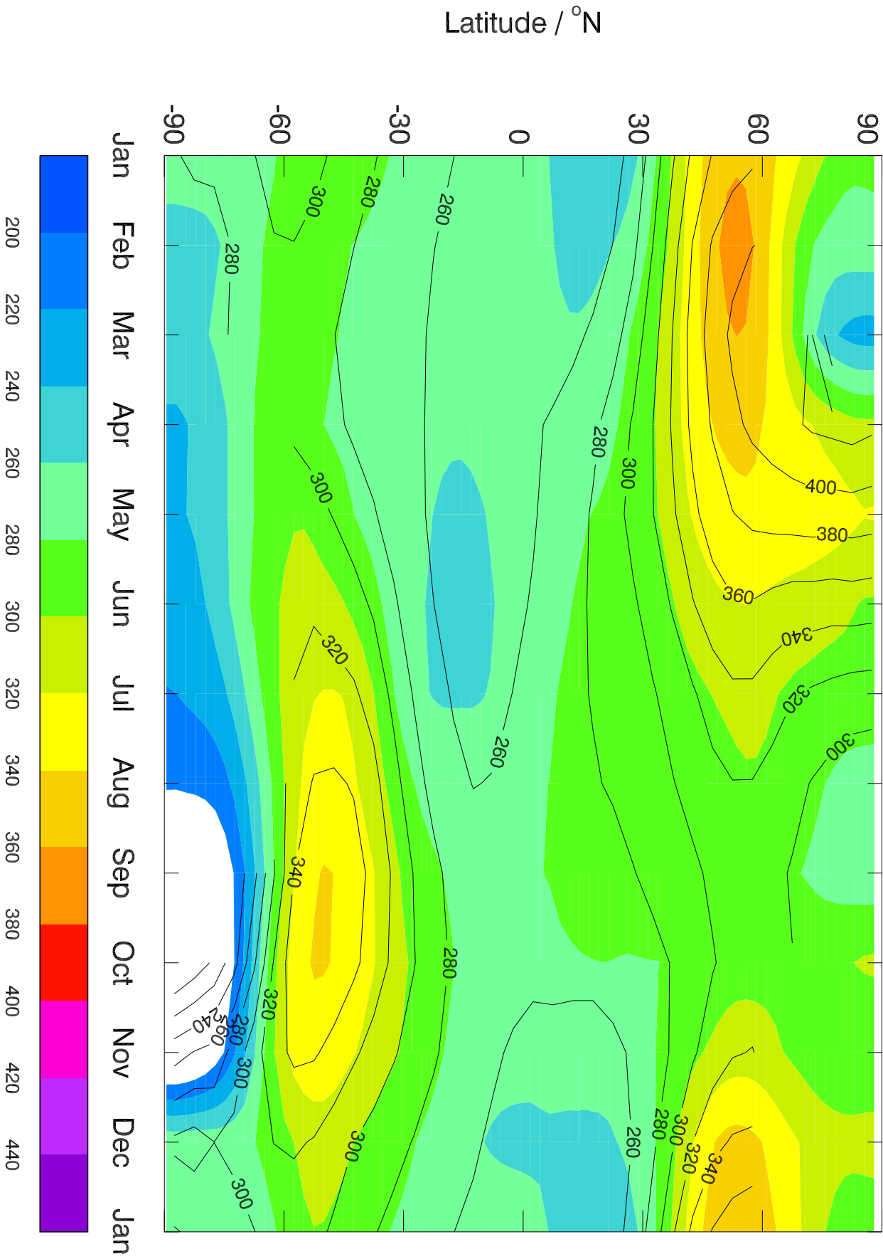
Total Ozone Column (DU). Colours: UKCA (XJCIR), Contours: TOMS
