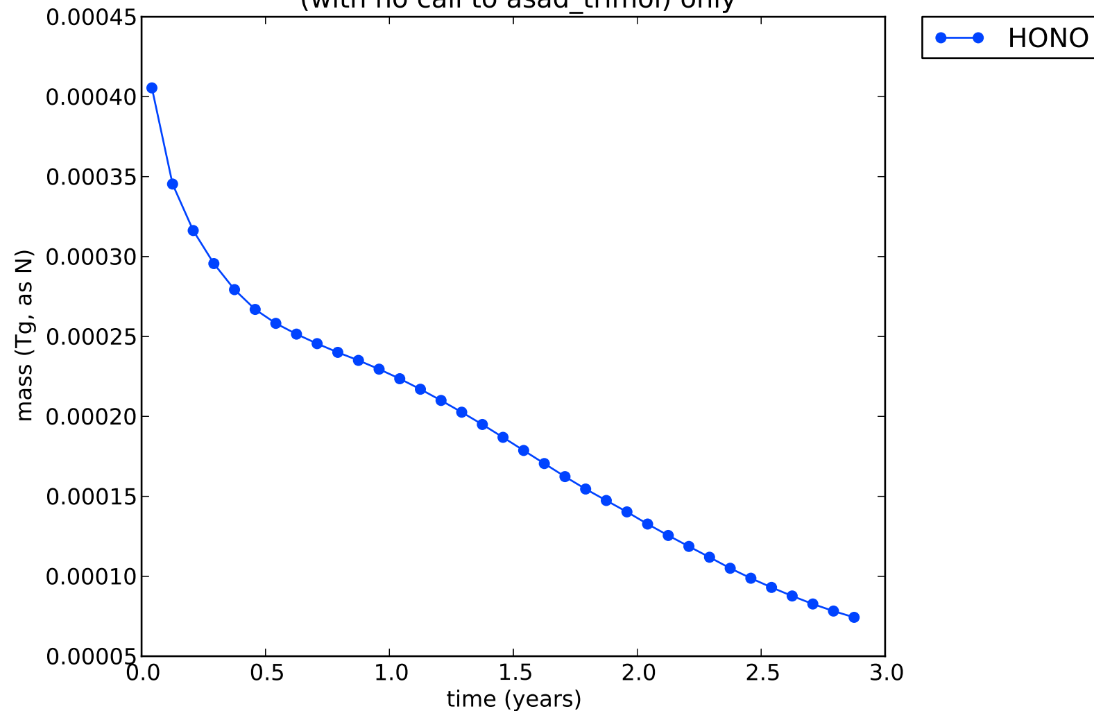
Call transform_halogen and chemistry_ctl (with no call to asad_trimol) only
