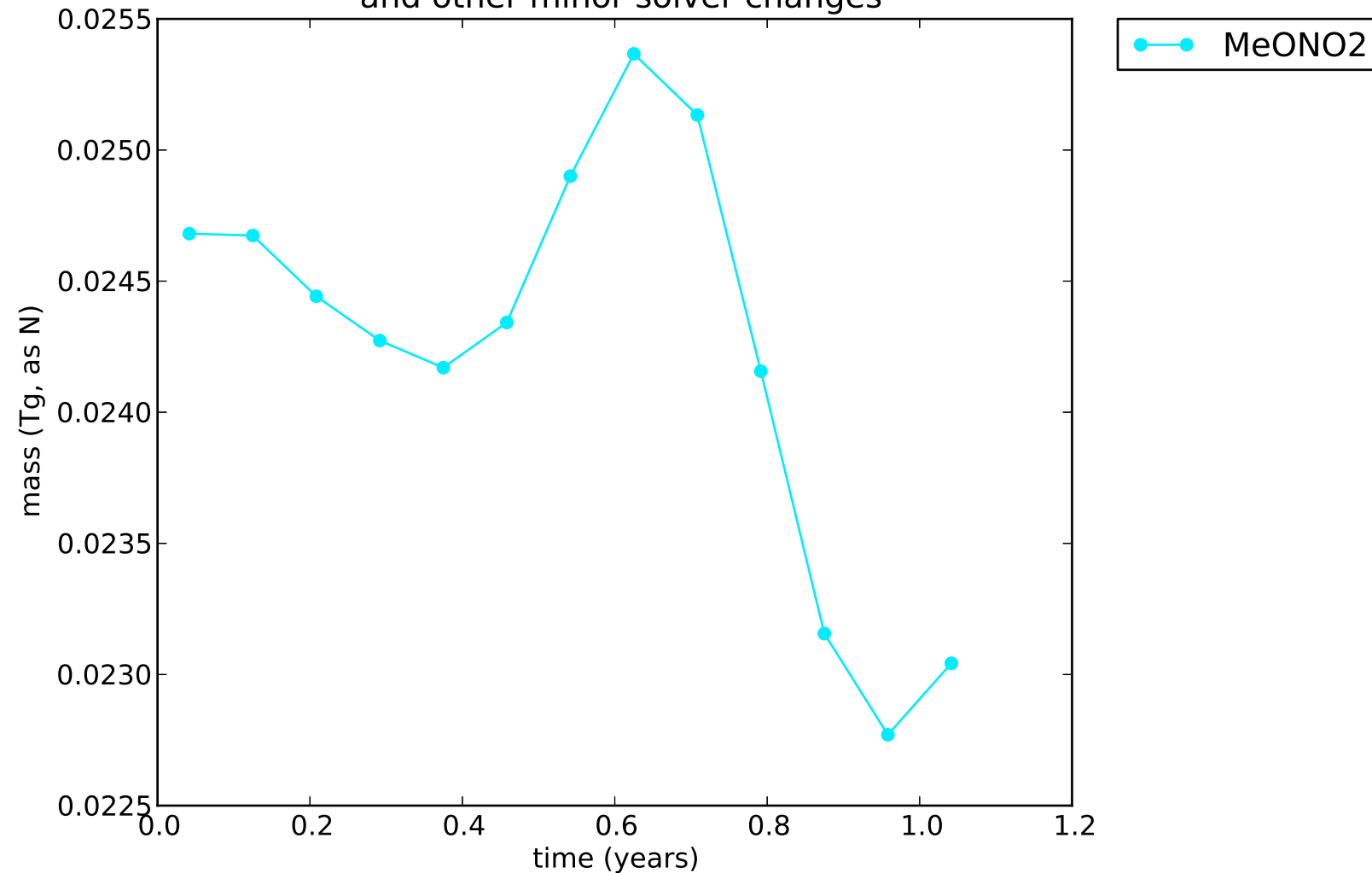
No prod/loss of NO y with 20min chemical timestep and other minor solver changes
