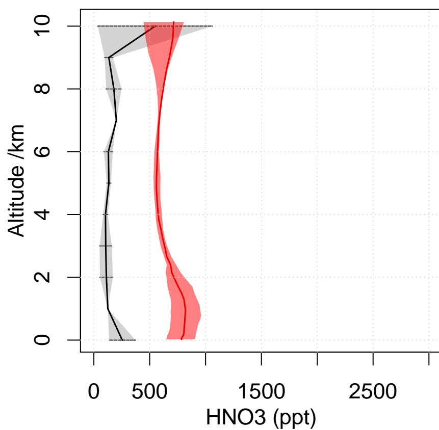
PEM-West-B Japan 1994 02 Lat 25 – 40 Lon 135 – 150
