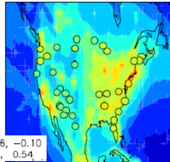
UKCA-UM Jun surface EC mass conc.
