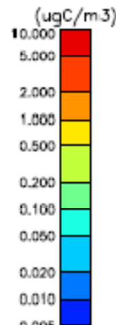
GLOMAP-mode Jun surface EC mass conc.
