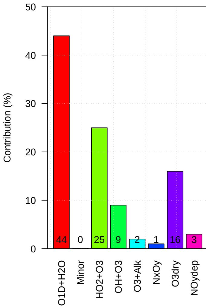
ao763 Loss of Tropospheric Ox
