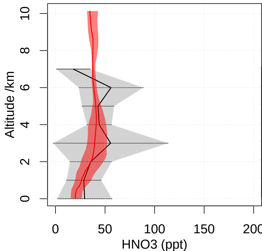
PEM-Tropics-B Christmas-Island 1999 01 Lat 0 – 10 Lon 200 – 220
