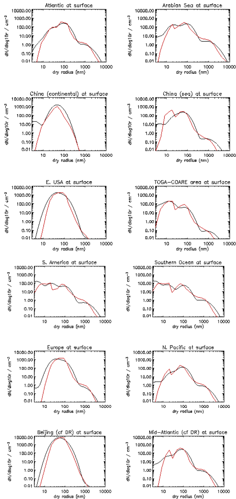
Figure 1 Annual mean size distributions ( dN/d\log_{10}r ) simulated by GLOMAP-mode (black) and GLOMAP-bin (red) at a variety of marine and continental surface locations.
