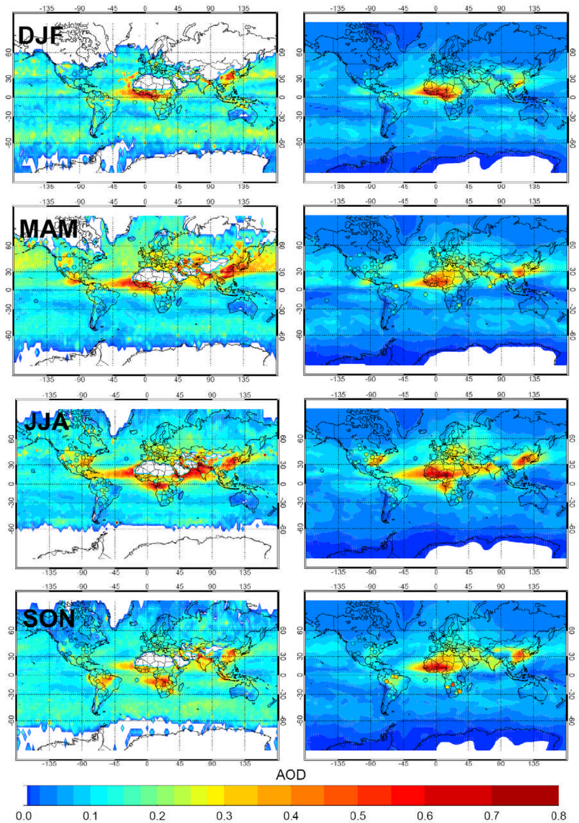
Figure 1 MODIS observed (left-hand panels) and GLOMAP-mode simulated (right-hand panels) 550nm Aerosol Optical Depth for year 2000 simulation. Filled circles indicate sun photometer observations at AERONET sites. Included in simulation are 7-modes containing sulphate, sea-salt, black carbon, organic carbon and dust).
