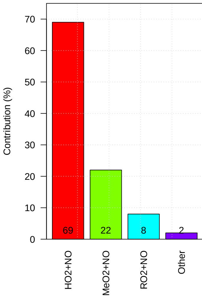
xhklm Production of Tropospheric Ox
