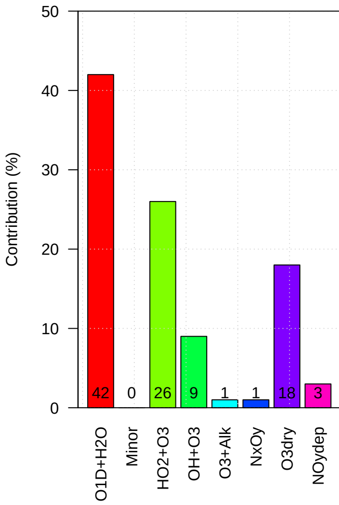
xhklm Loss of Tropospheric Ox
