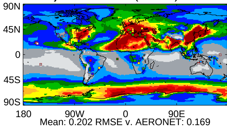
xjcih Total AOD (440nm) JJA
