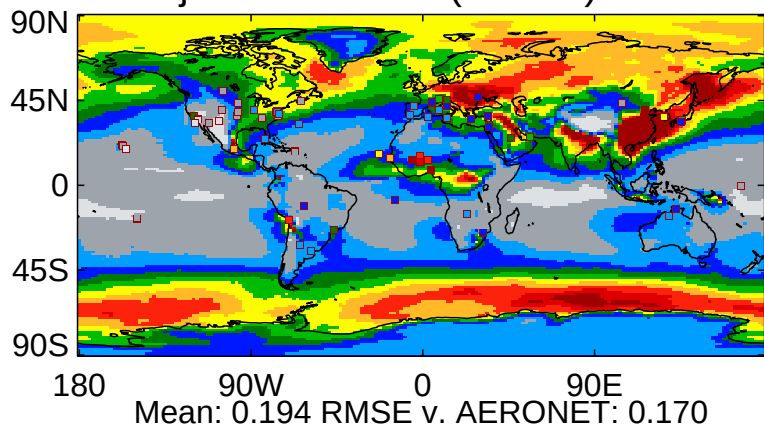
xjcih Total AOD (440nm) DJF
