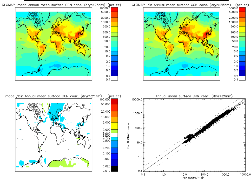
Figure 1: Simulated annual mean surface cloud condensation nuclei concentrations in GLOMAP-mode (top-left) and GLOMAP-bin (top right). The ratio of GLOMAP-mode to GLOMAP-bin simulated CCN concentration is shown in the bottom left plot.
