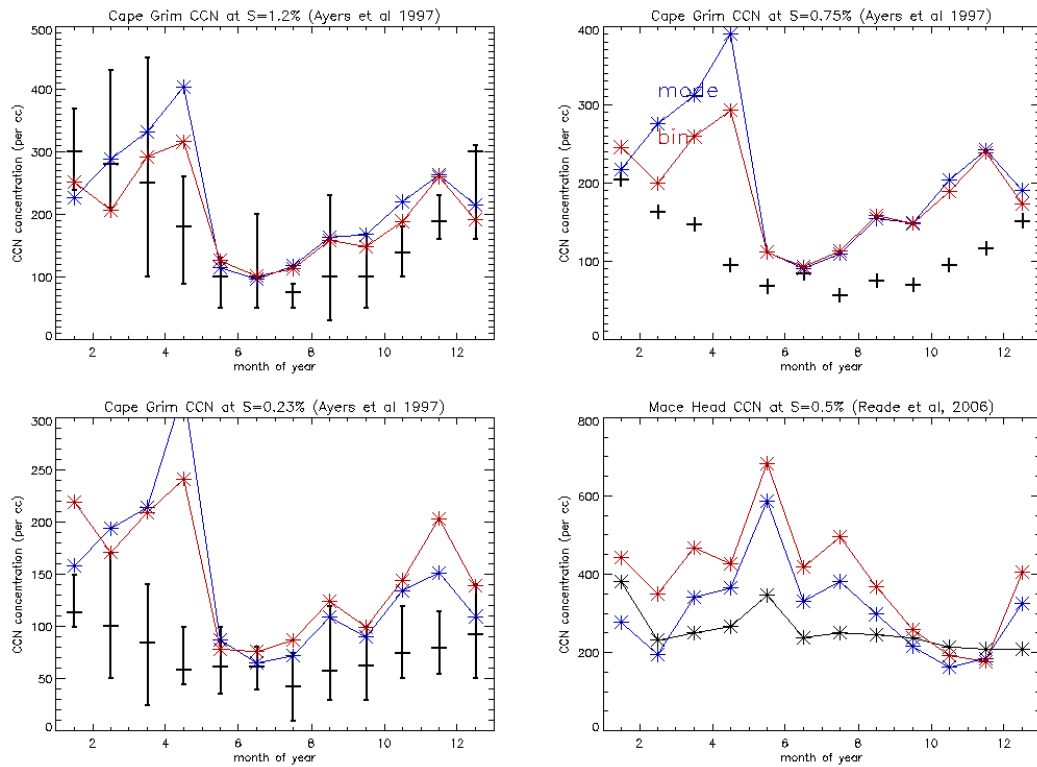
Figure 2 Annual cycle of GLOMAP-mode simulated (blue) monthly mean CCN concentrations against observations (black) and simulated by GLOMAP-bin (red). Cape Grim CCN are at 0.23 (bottom left), 0.75 (top right), 1.2% (top left) supersaturation
