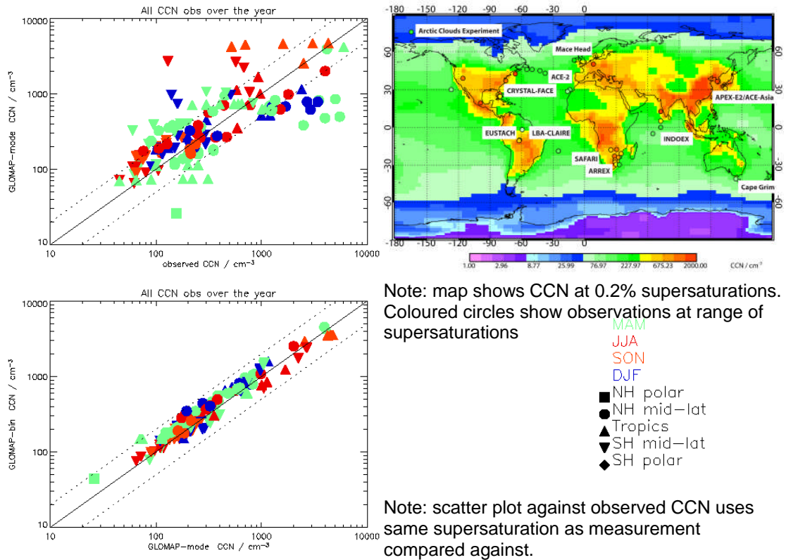
Figure 1 GLOMAP-mode simulated monthly-mean surface CCN concentrations compared to that observed from a range of fields campaigns (see top right plot) and monitoring sites (top left plot) and that simulated by GLOMAP-bin (bottom left plot).
