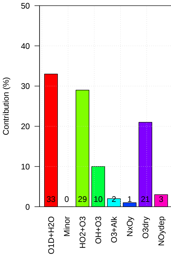
ajkzh Loss of Tropospheric Ox
