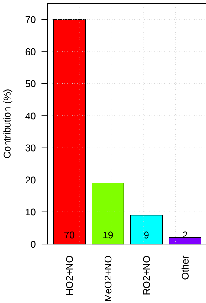
ajkzh Production of Tropospheric Ox
