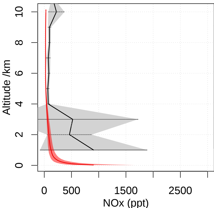
TRACE-A S-Africa 1992 09 Lat -25 – -5 Lon 15 – 35
