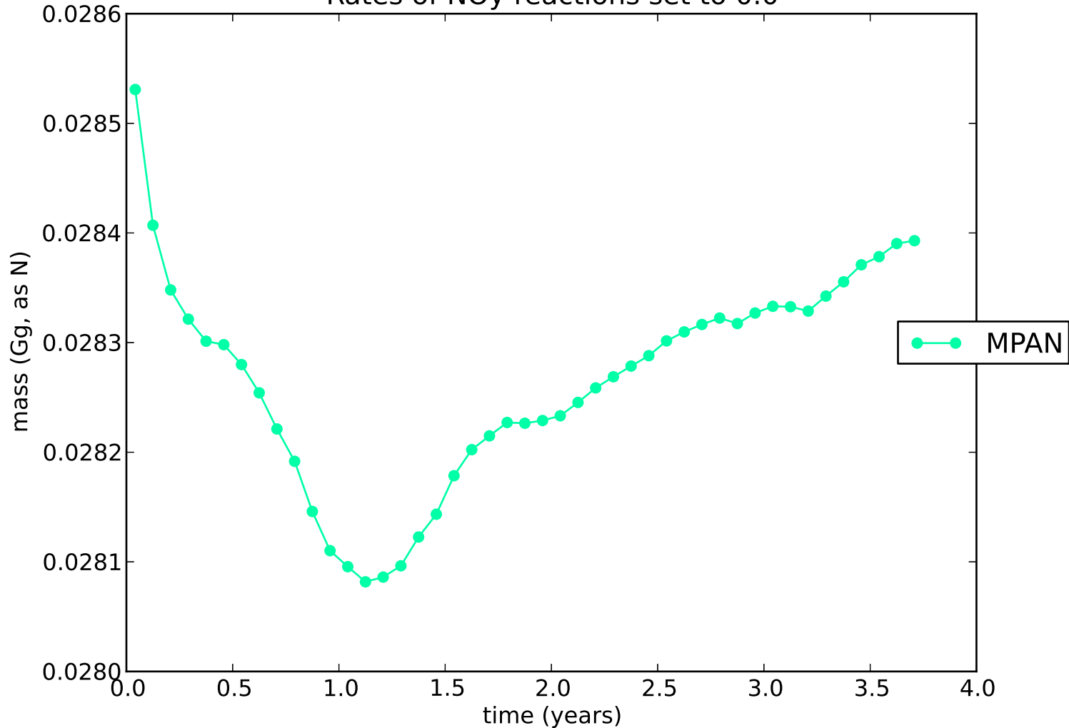
Rates of NO y reactions set to 0.0
