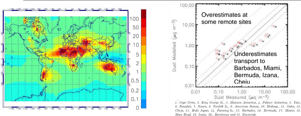
Figure 1: Global map and scatter of simulated annual mean surface dust mass concentrations vs observations from the global University of Miami monitoring network.
