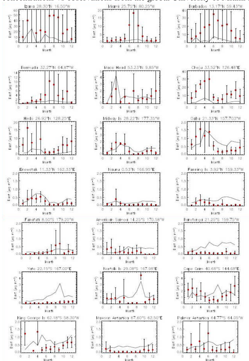
Figure 2: Plots of simulated annual cycle monthly-mean mean surface dust mass concentrations vs observations from the global University of Miami monitoring network.
