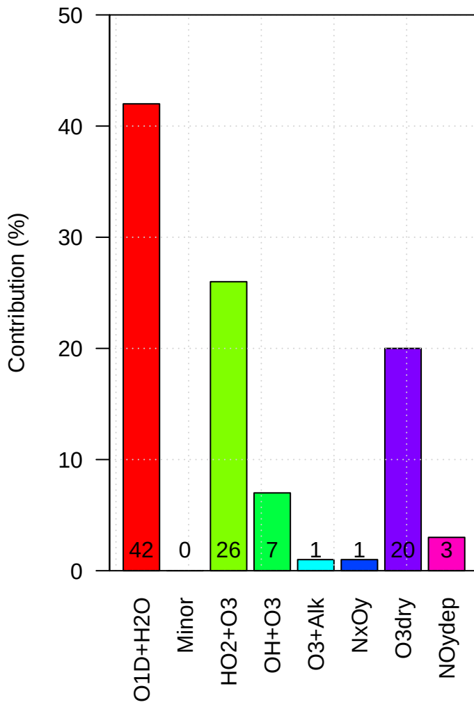
xjcih Loss of Tropospheric Ox
