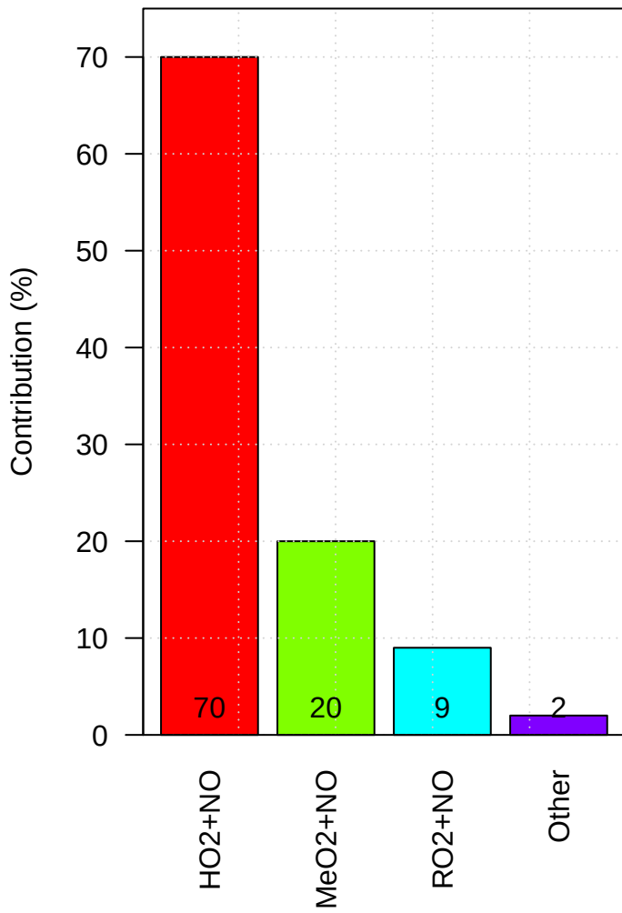
xjcih Production of Tropospheric Ox
