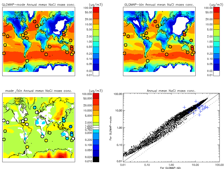
Figure 2: Simulated annual mean surface NaCl against U. Miami observations (global) N.b. black dots in scatterplot show GLOMAP-mode vs GLOMAP-bin comparison. Light blue pluses in scatter plot indicate GLOMAP-mode vs U. Miami observations. Lower left plot shows GLOMAP-mode divided by GLOMAP-bin simulated mass.
