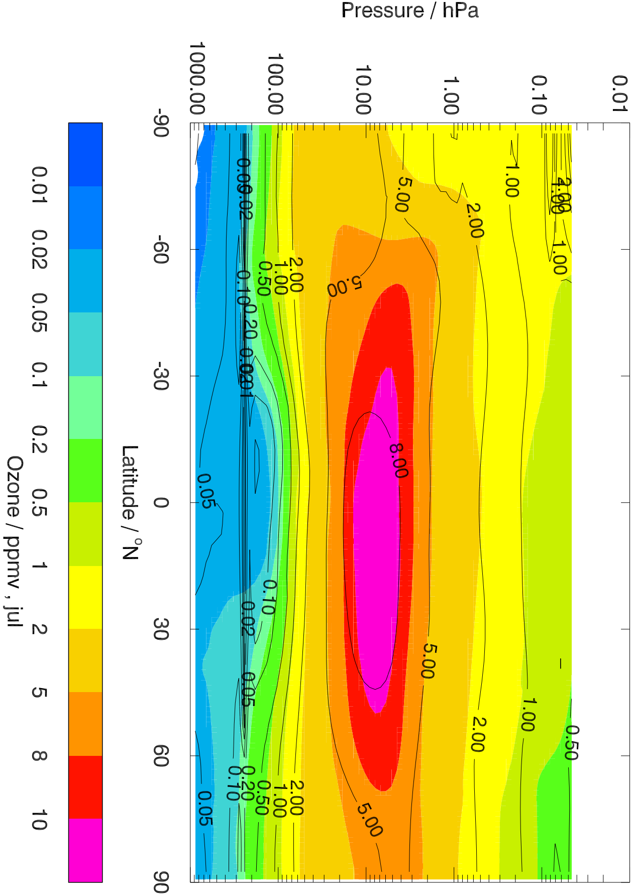
Colours: UKCA (XJCL), Contours: NIWA-CCMVal
