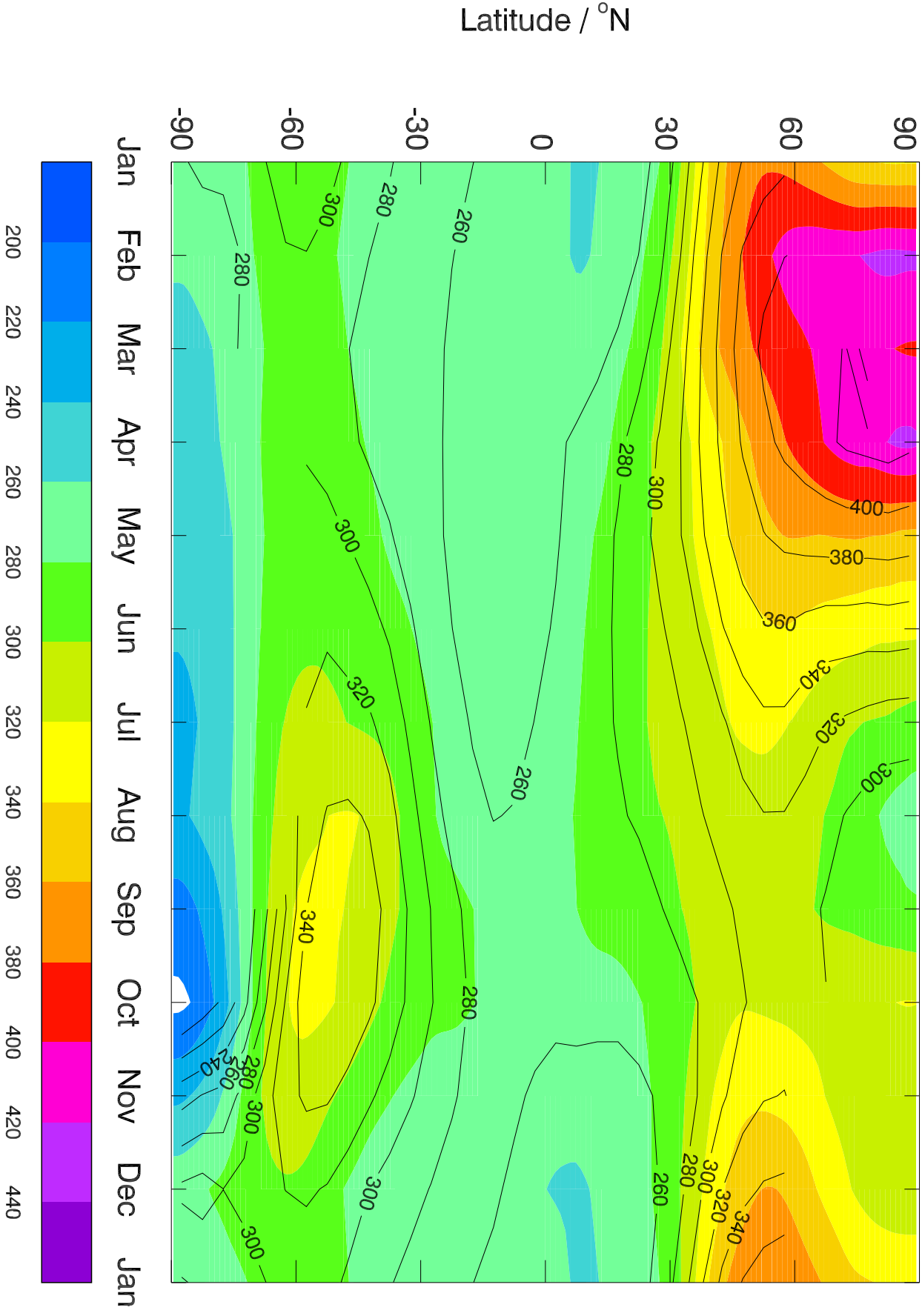
Total Ozone Column (DU). Colours: UKCA (XJcIL), Contours: TOMS
