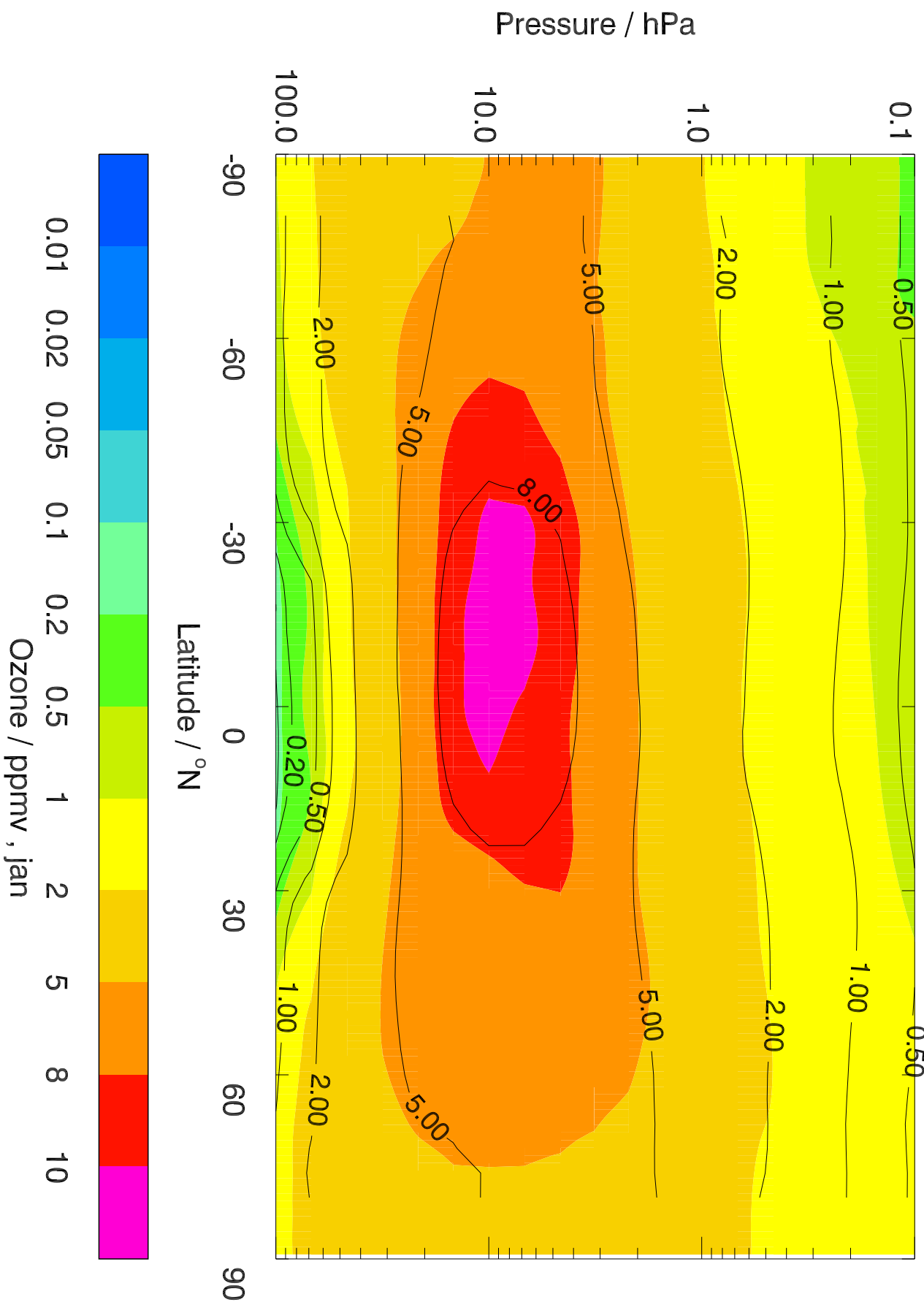
Colours: UKCA (XHKLS), Contours: HALOE
