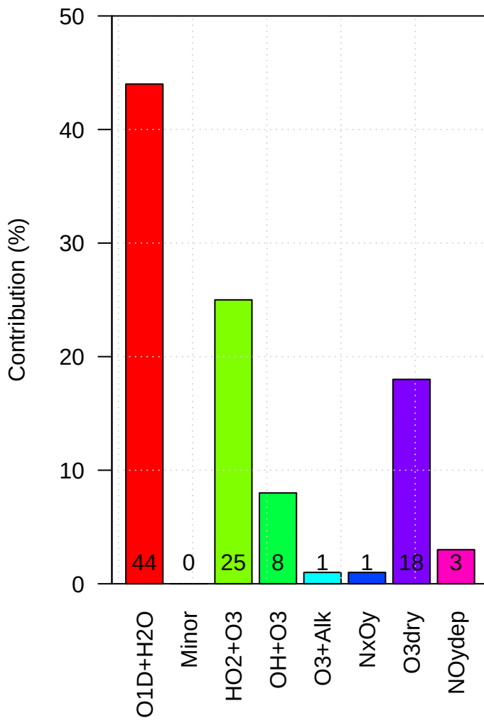
xhkl's Loss of Tropospheric Ox
