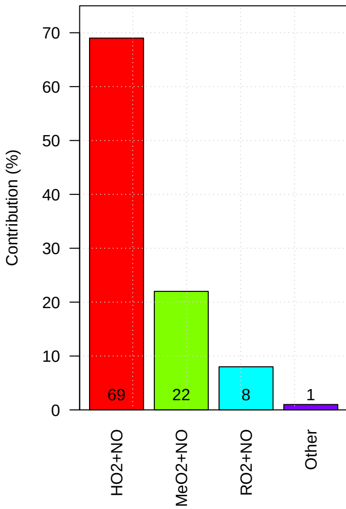
xhkl's Production of Tropospheric Ox
