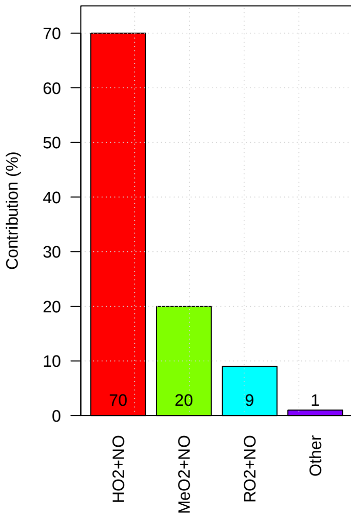
xjcij Production of Tropospheric Ox
