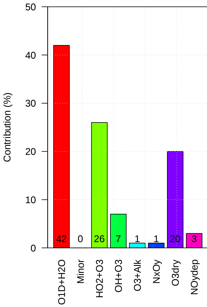
xjcij Loss of Tropospheric Ox
