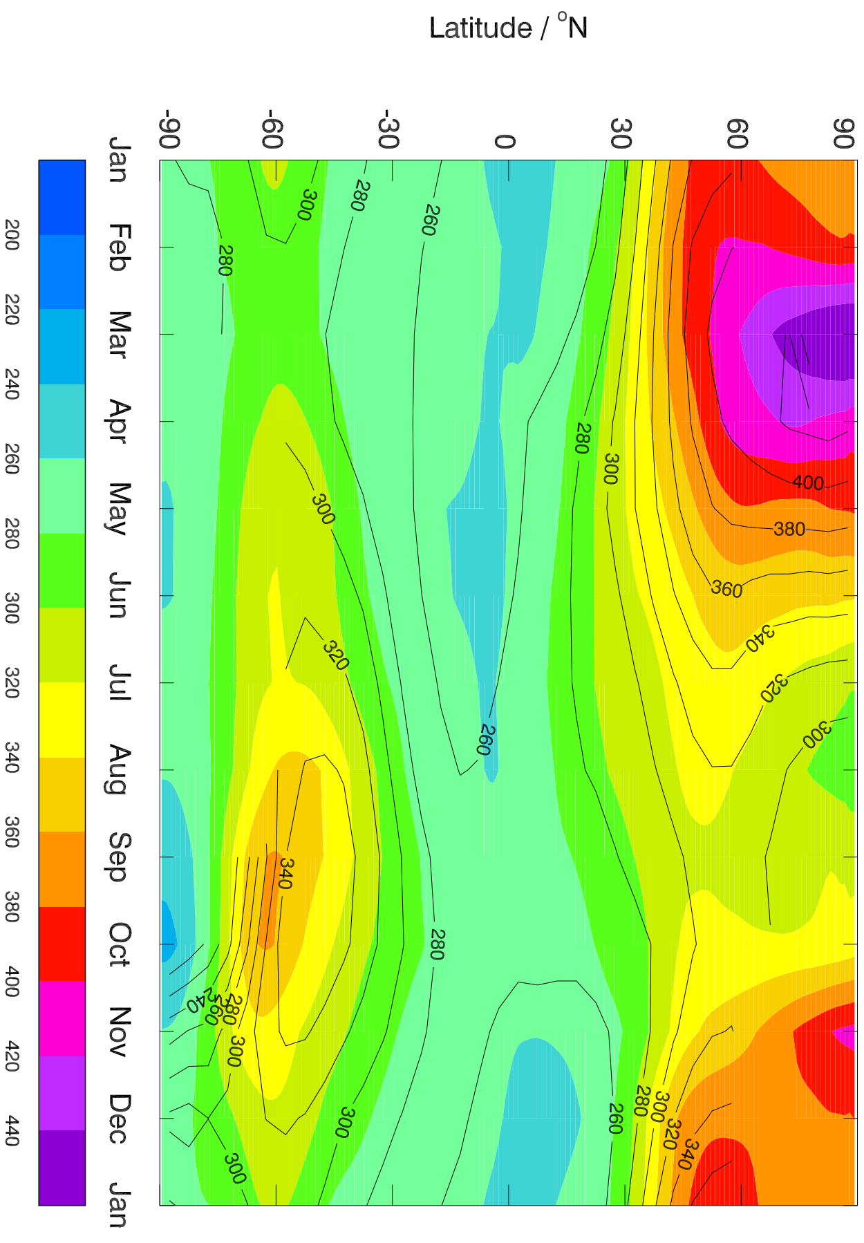
Total Ozone Column (DU). Colours: UKCA (XJCIJ), Contours: TOMS
