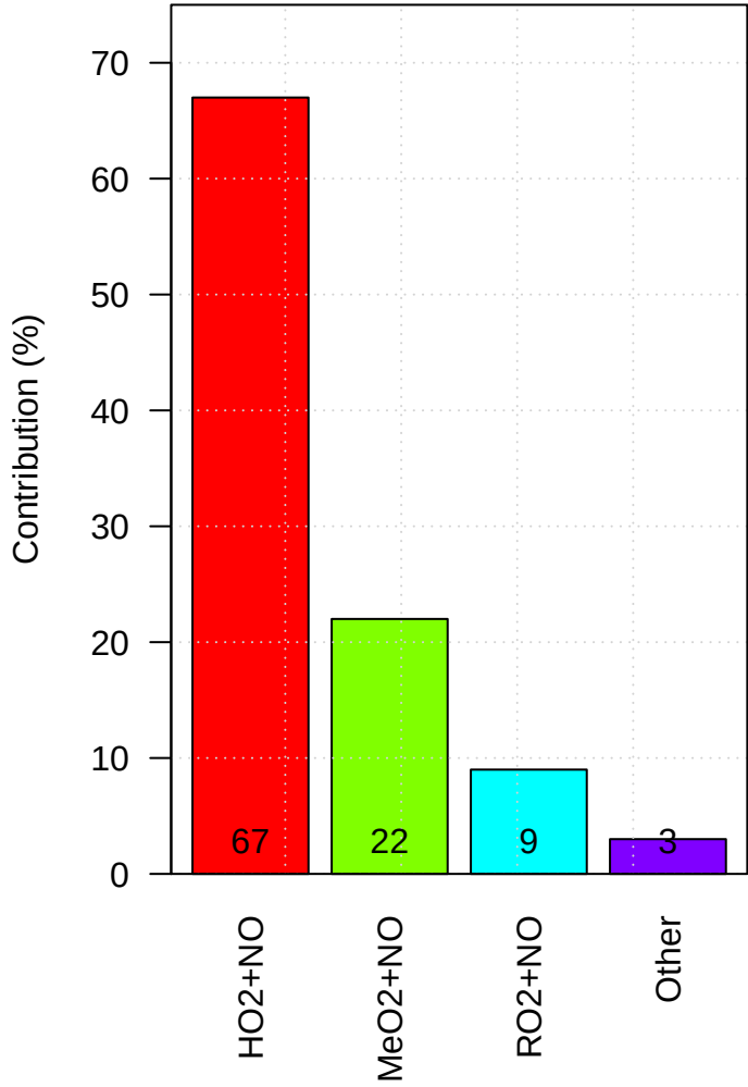
ameku Production of Tropospheric Ox
