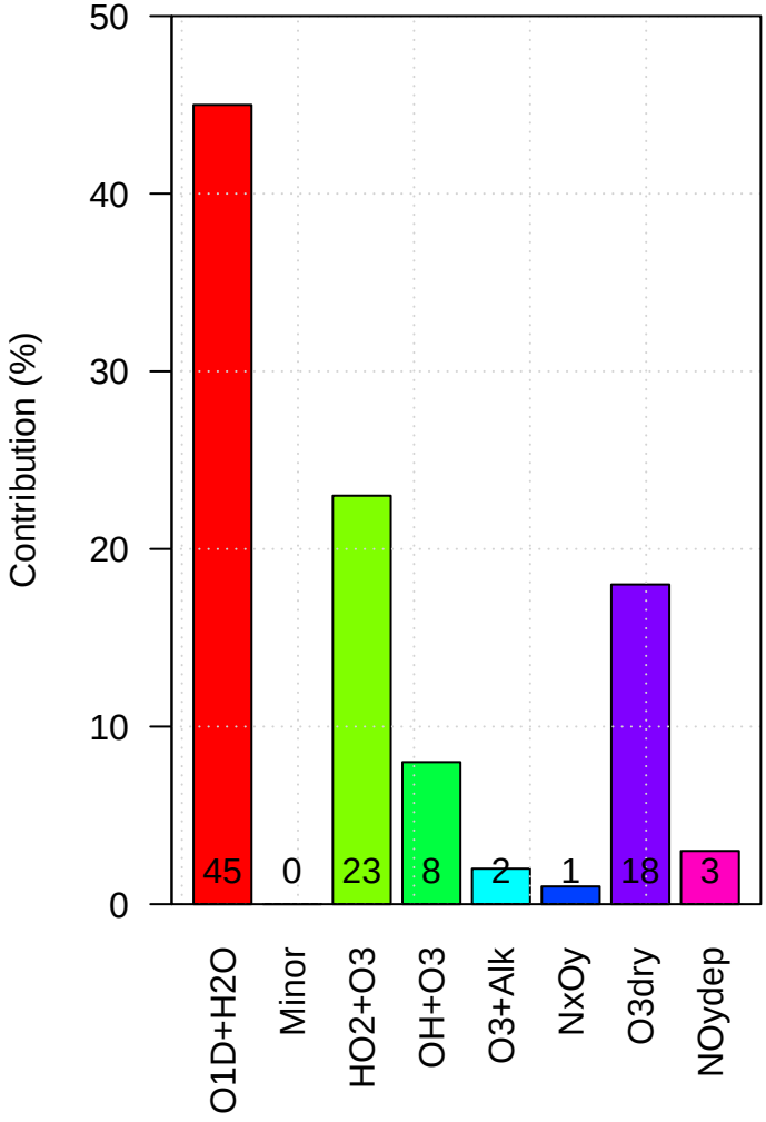
ameku Loss of Tropospheric Ox
