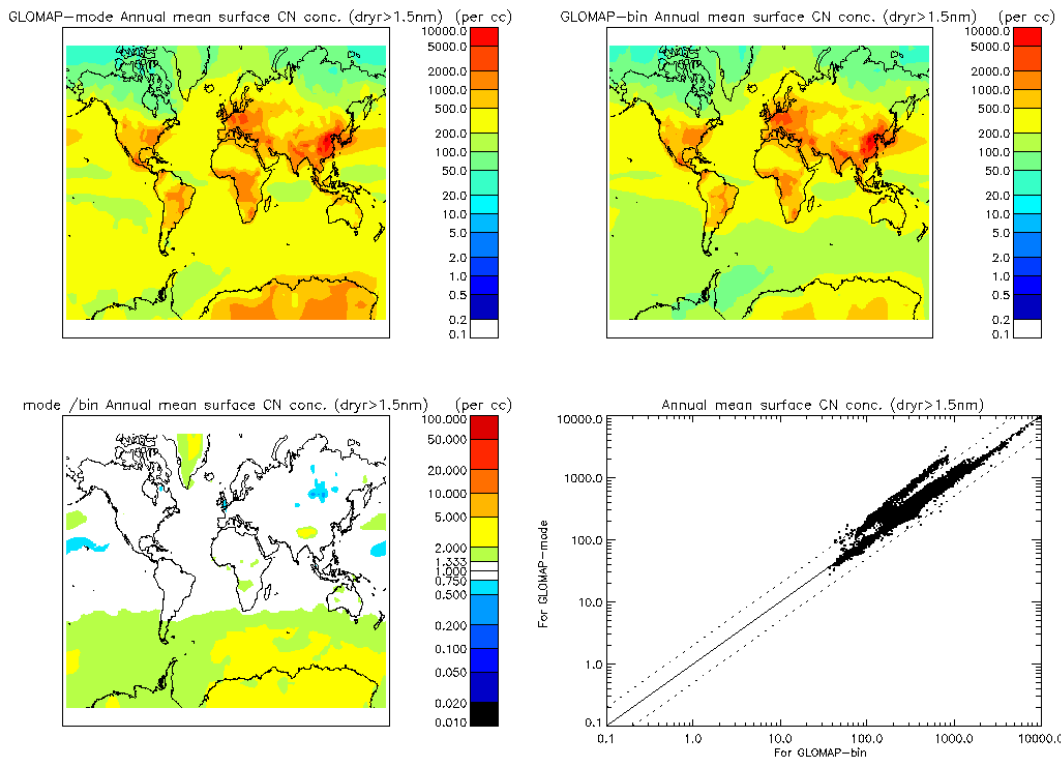
Figure 1: Simulated annual mean surface condensation nuclei concentrations in GLOMAP-mode (top-left) and GLOMAP-bin (top right). The ratio of GLOMAP-mode to GLOMAP-bin simulated CN concentration is shown in the bottom left plot. N.b. black dots in scatterplot (bottom right) show GLOMAP-mode vs GLOMAP-bin.
