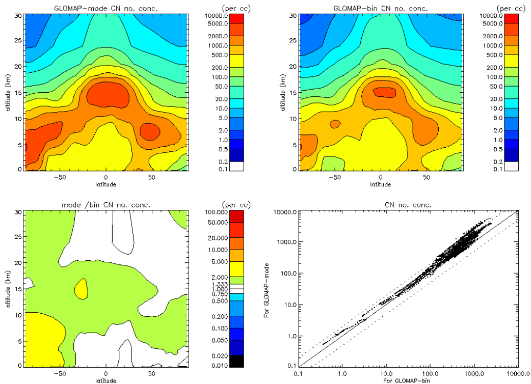
Figure 2: Simulated annual zonal mean condensation nuclei concentrations in GLOMAP-mode (top-left) and GLOMAP-bin (top right). The ratio of GLOMAP-mode to GLOMAP-bin simulated CN concentration is shown in the bottom left plot. N.b. black dots in scatterplot (bottom right) show GLOMAP-mode vs GLOMAP-bin.
