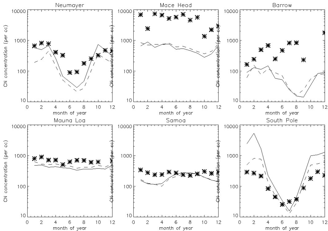
Figure 2 Observed monthly-mean (*) surface CN concentrations at 6 GAW monitoring stations compared to that simulated by GLOMAP-mode (solid) and -bin (dashed)
