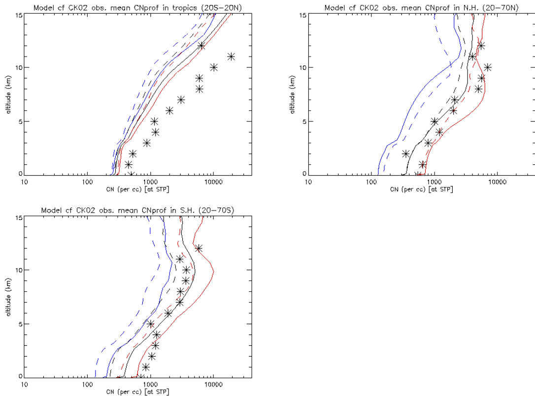
Figure 1 Observed climatology of profiles of CN concentrations (at s.t.p.) over the Pacific Ocean (Clarke & Kapustin, 2002) against that simulated by GLOMAP-mode (solid lines) and GLOMAP-bin (dashed lines). Black lines indicate annual mean profile, blue (red) indicate minimum (maximum) monthly-mean simulated CN at each height.
